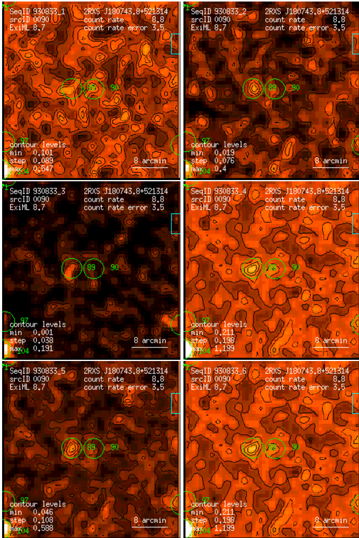
Figure 90: RASS 930833: detection 0090: band rate images, Gaussian filter: (1) PSPC channels 11 – 41, (2) 52 – 90, (3) 91 – 201, (4) 11 – 235, (5) 52 – 201, (6) 11 – 201. Broad band rates in counts/ks. Band rate contour levels in counts/ks/arcmin 2 .
