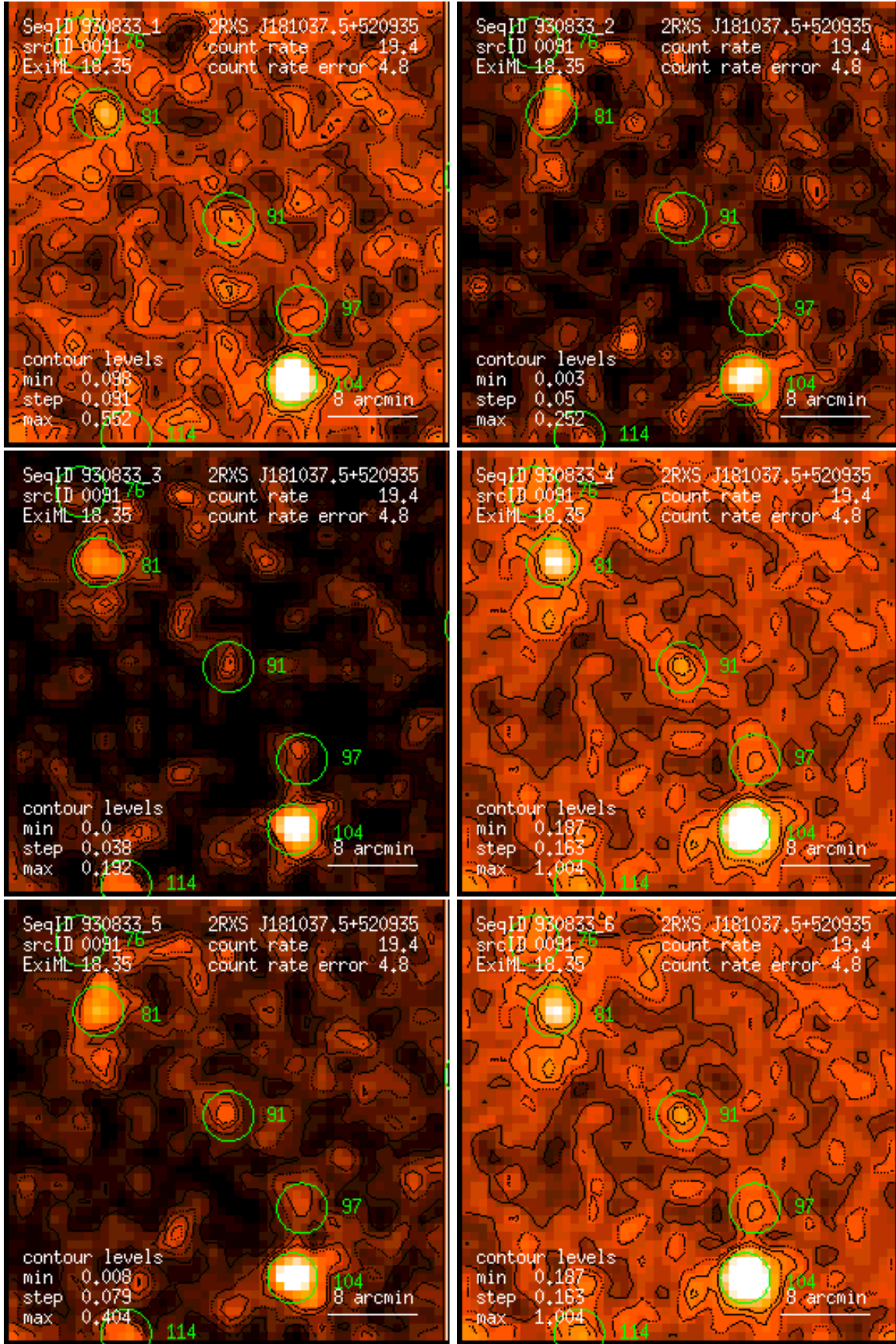
Figure 91: RASS 930833: detection 0091: band rate images, Gaussian filter: (1) PSPC channels 11 – 41, (2) 52 – 90, (3) 91 – 201, (4) 11 – 235, (5) 52 – 201, (6) 11 – 201. Broad band rates in counts/ks. Band rate contour levels in counts/ks/arcmin 2 .
