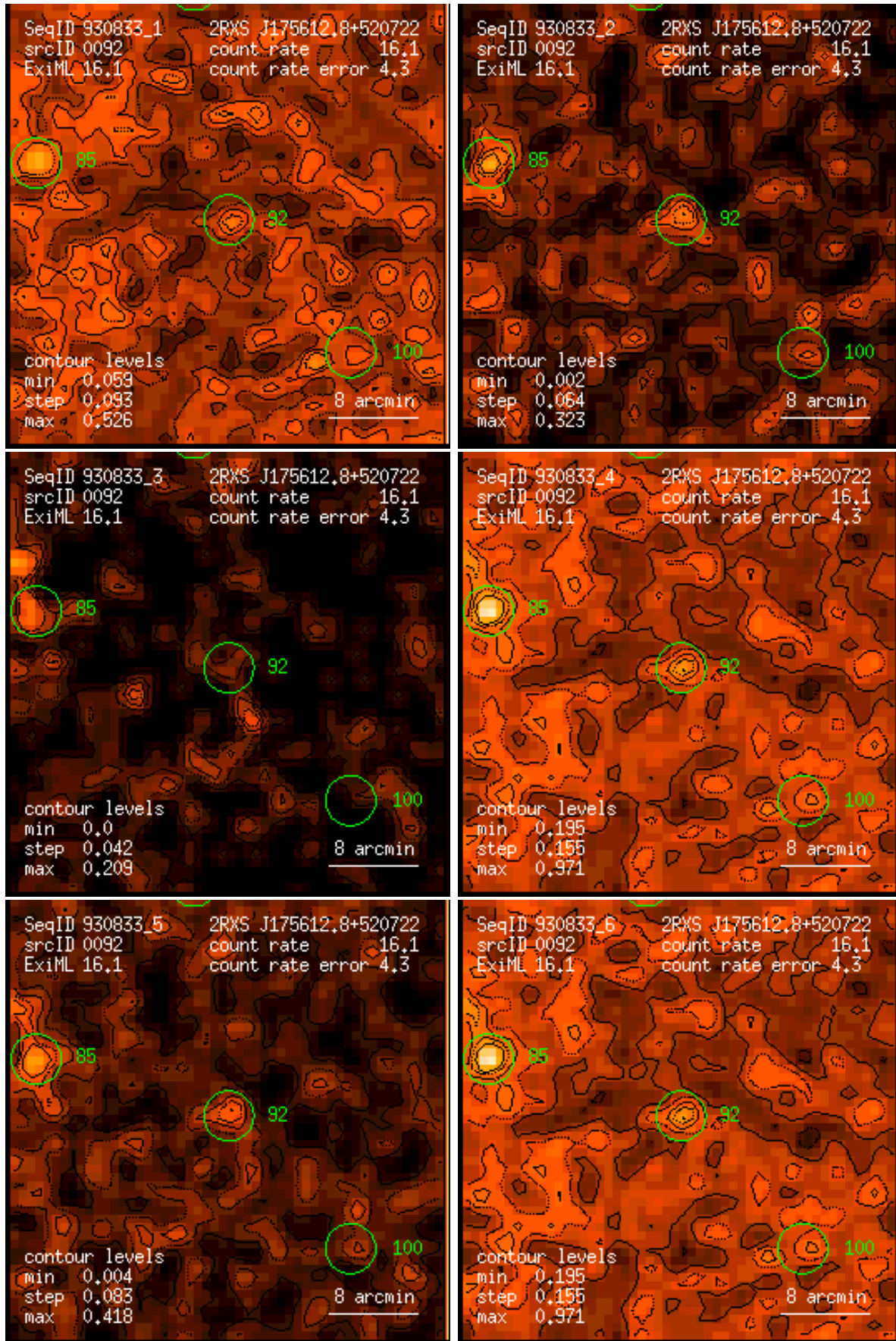
Figure 92: RASS 930833: detection 0092: band rate images, Gaussian filter: (1) PSPC channels 11 – 41, (2) 52 – 90, (3) 91 – 201, (4) 11 – 235, (5) 52 – 201, (6) 11 – 201. Broad band rates in counts/ks. Band rate contour levels in counts/ks/arcmin 2 .
