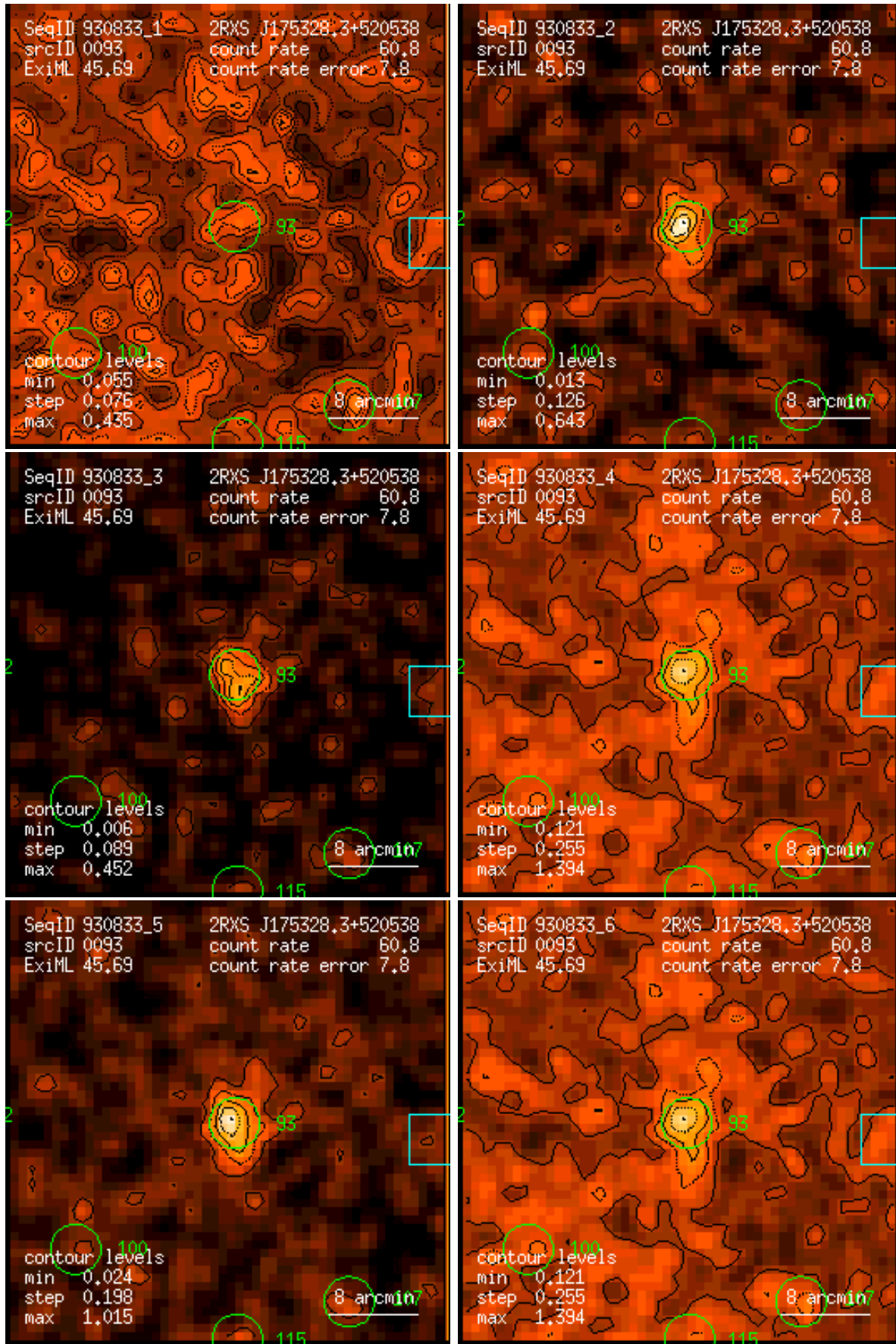
Figure 93: RASS 930833: detection 0093: band rate images, Gaussian filter: (1) PSPC channels 11 – 41, (2) 52 – 90, (3) 91 – 201, (4) 11 – 235, (5) 52 – 201, (6) 11 – 201. Broad band rates in counts/ks. Band rate contour levels in counts/ks/arcmin 2 .
