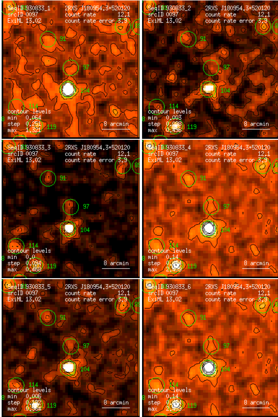
Figure 97: RASS 930833: detection 0097: band rate images, Gaussian filter: (1) PSPC channels 11 – 41, (2) 52 – 90, (3) 91 – 201, (4) 11 – 235, (5) 52 – 201, (6) 11 – 201. Broad band rates in counts/ks. Band rate contour levels in counts/ks/arcmin 2 .
