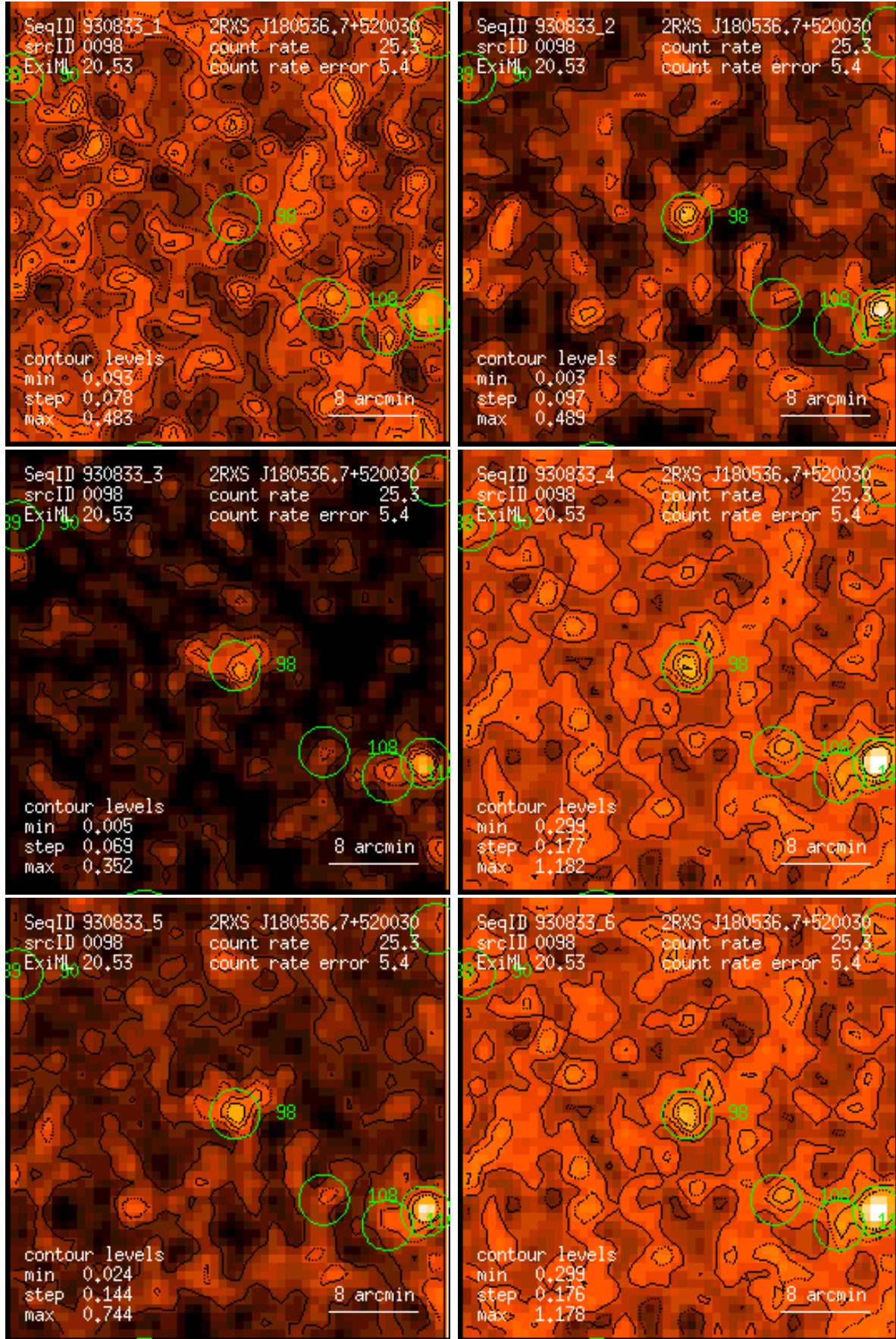
Figure 98: RASS 930833: detection 0098: band rate images, Gaussian filter: (1) PSPC channels 11 – 41, (2) 52 – 90, (3) 91 – 201, (4) 11 – 235, (5) 52 – 201, (6) 11 – 201. Broad band rates in counts/ks. Band rate contour levels in counts/ks/arcmin 2 .
