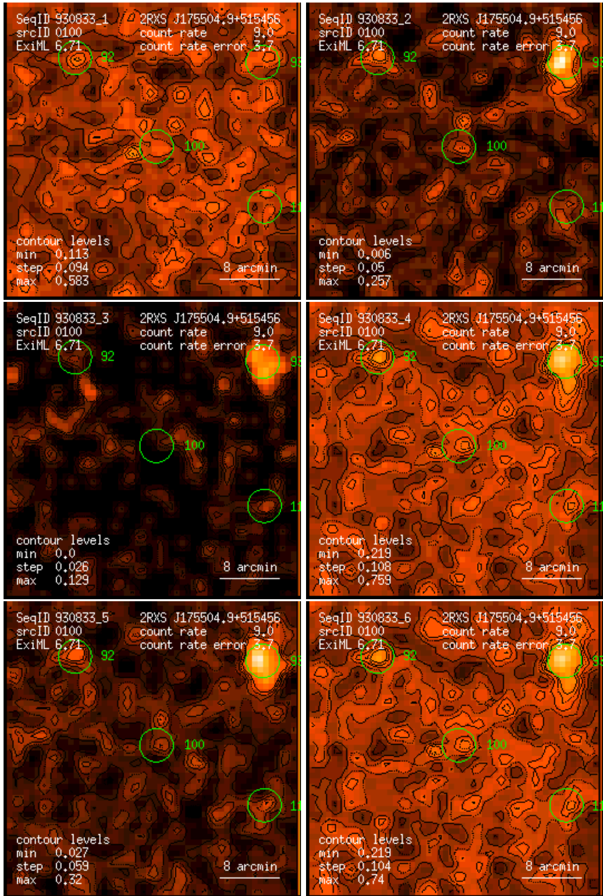
Figure 100: RASS 930833: detection 0100: band rate images, Gaussian filter: (1) PSPC channels 11 – 41, (2) 52 – 90, (3) 91 – 201, (4) 11 – 235, (5) 52 – 201, (6) 11 – 201. Broad band rates in counts/ks. Band rate contour levels in counts/ks/arcmin 2 .
