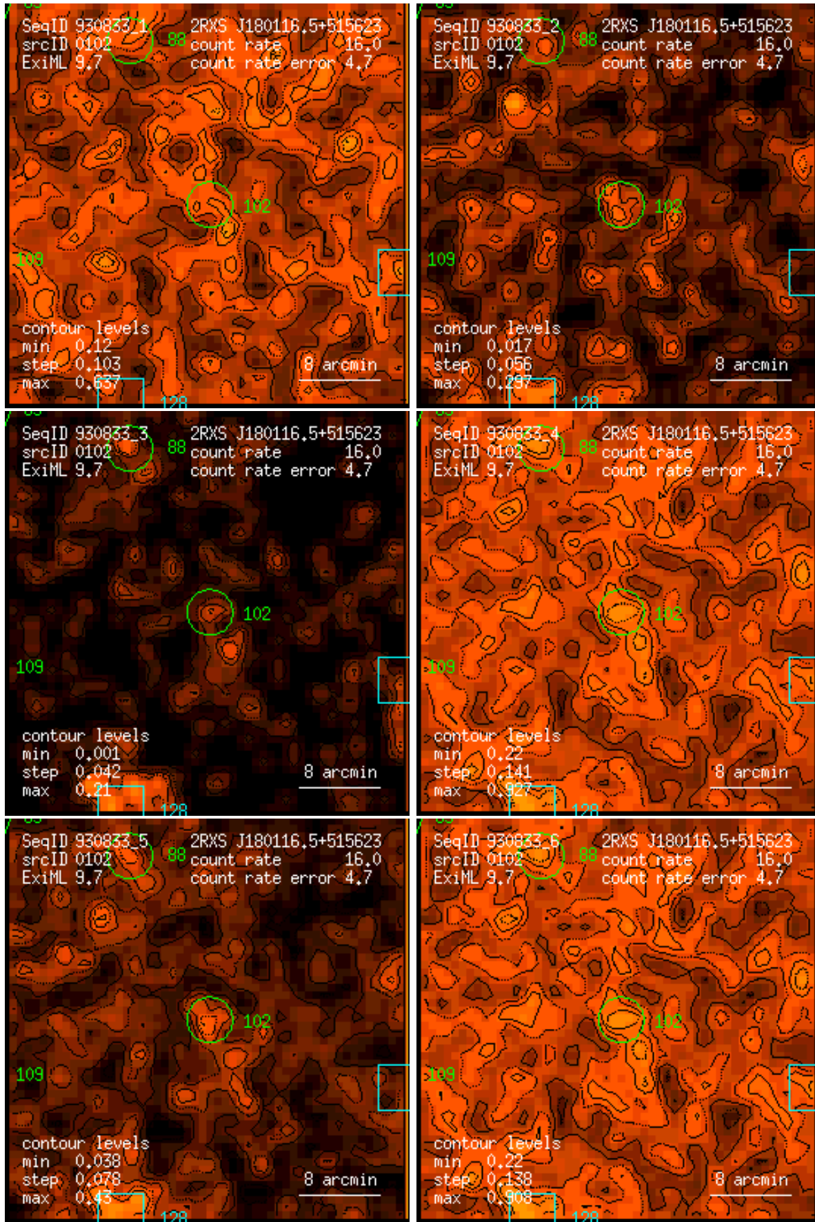
Figure 102: RASS 930833: detection 0102: band rate images, Gaussian filter: (1) PSPC channels 11 – 41, (2) 52 – 90, (3) 91 – 201, (4) 11 – 235, (5) 52 – 201, (6) 11 – 201. Broad band rates in counts/ks. Band rate contour levels in counts/ks/arcmin 2 .
