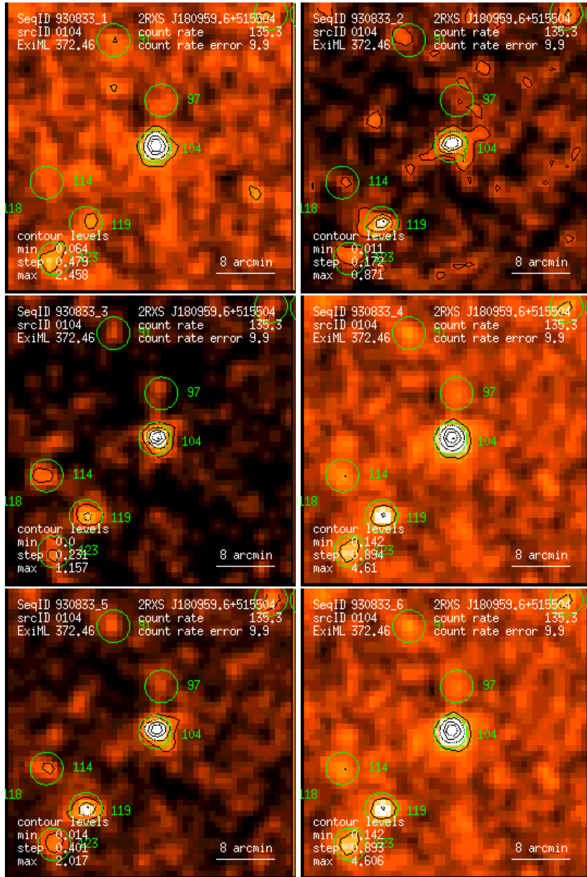
Figure 104: RASS 930833: detection 0104: band rate images, Gaussian filter: (1) PSPC channels 11 – 41, (2) 52 – 90, (3) 91 – 201, (4) 11 – 235, (5) 52 – 201, (6) 11 – 201. Broad band rates in counts/ks. Band rate contour levels in counts/ks/arcmin 2 .
