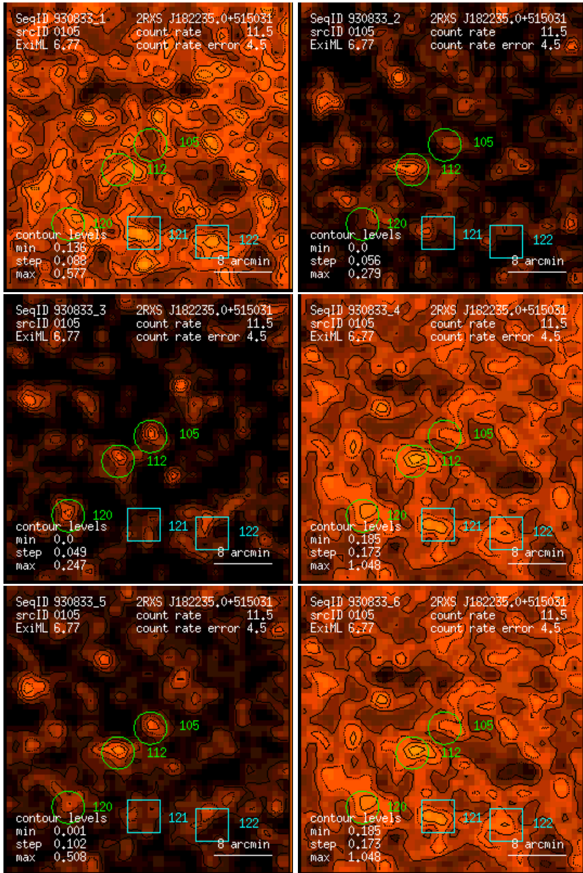
Figure 105: RASS 930833: detection 0105: band rate images, Gaussian filter: (1) PSPC channels 11 – 41, (2) 52 – 90, (3) 91 – 201, (4) 11 – 235, (5) 52 – 201, (6) 11 – 201. Broad band rates in counts/ks. Band rate contour levels in counts/ks/arcmin 2 .
