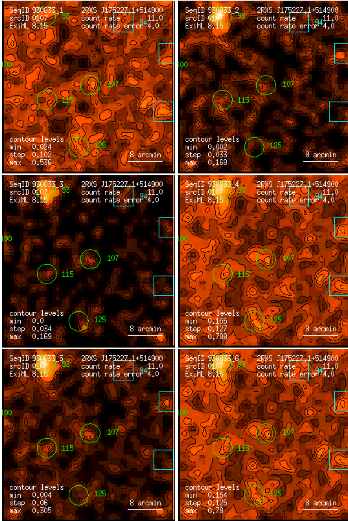
Figure 107: RASS 930833: detection 0107: band rate images, Gaussian filter: (1) PSPC channels 11 – 41, (2) 52 – 90, (3) 91 – 201, (4) 11 – 235, (5) 52 – 201, (6) 11 – 201. Broad band rates in counts/ks. Band rate contour levels in counts/ks/arcmin 2 .
