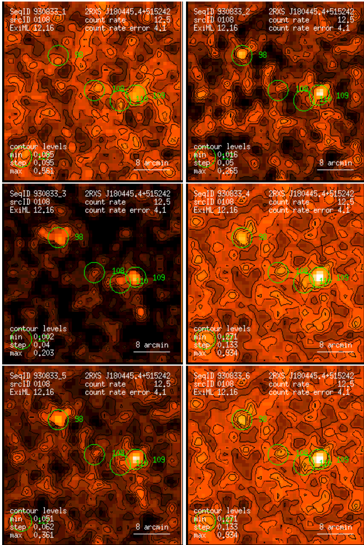
Figure 108: RASS 930833: detection 0108: band rate images, Gaussian filter: (1) PSPC channels 11 – 41, (2) 52 – 90, (3) 91 – 201, (4) 11 – 235, (5) 52 – 201, (6) 11 – 201. Broad band rates in counts/ks. Band rate contour levels in counts/ks/arcmin 2 .
