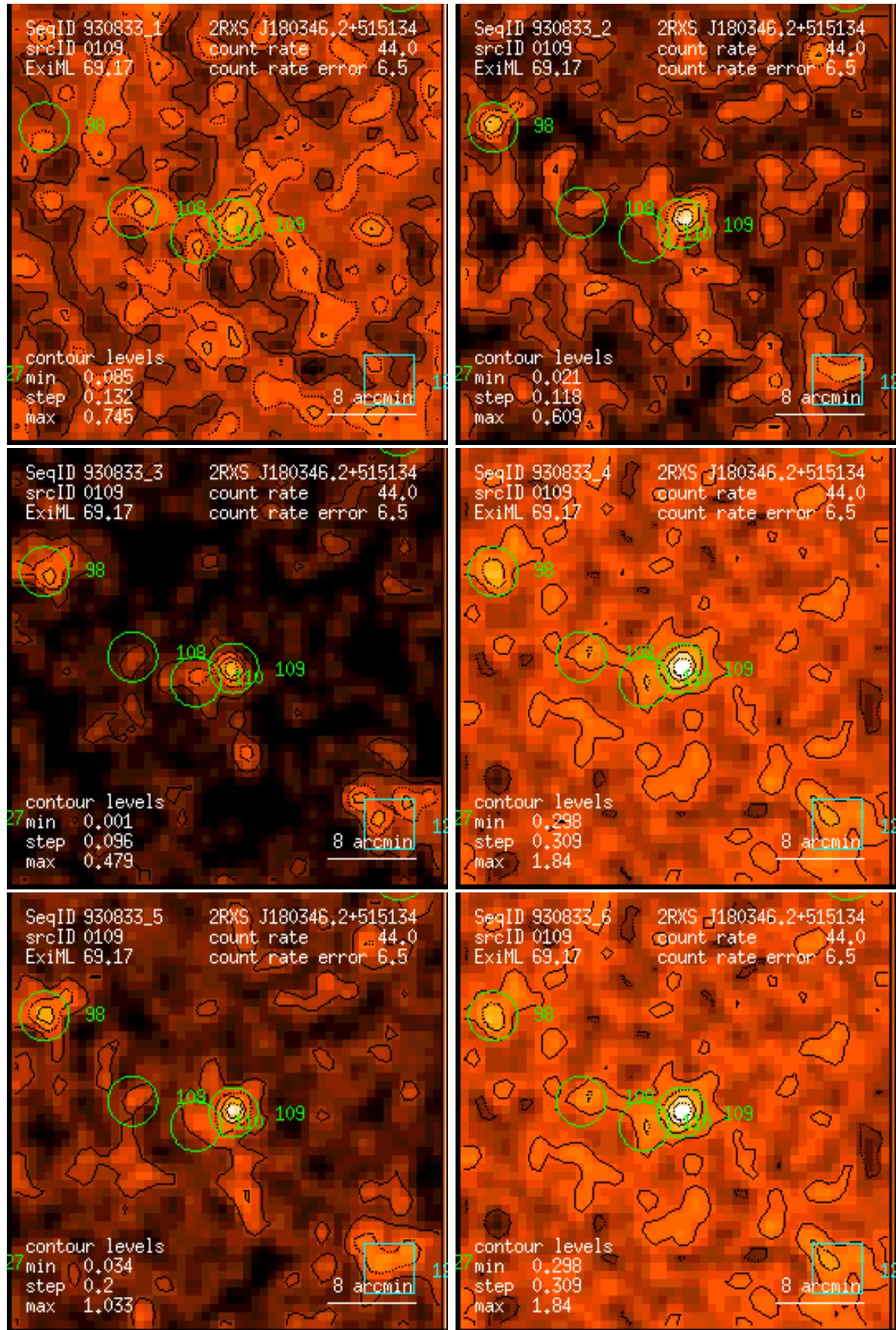
Figure 109: RASS 930833: detection 0109: band rate images, Gaussian filter: (1) PSPC channels 11 – 41, (2) 52 – 90, (3) 91 – 201, (4) 11 – 235, (5) 52 – 201, (6) 11 – 201. Broad band rates in counts/ks. Band rate contour levels in counts/ks/arcmin 2 .
