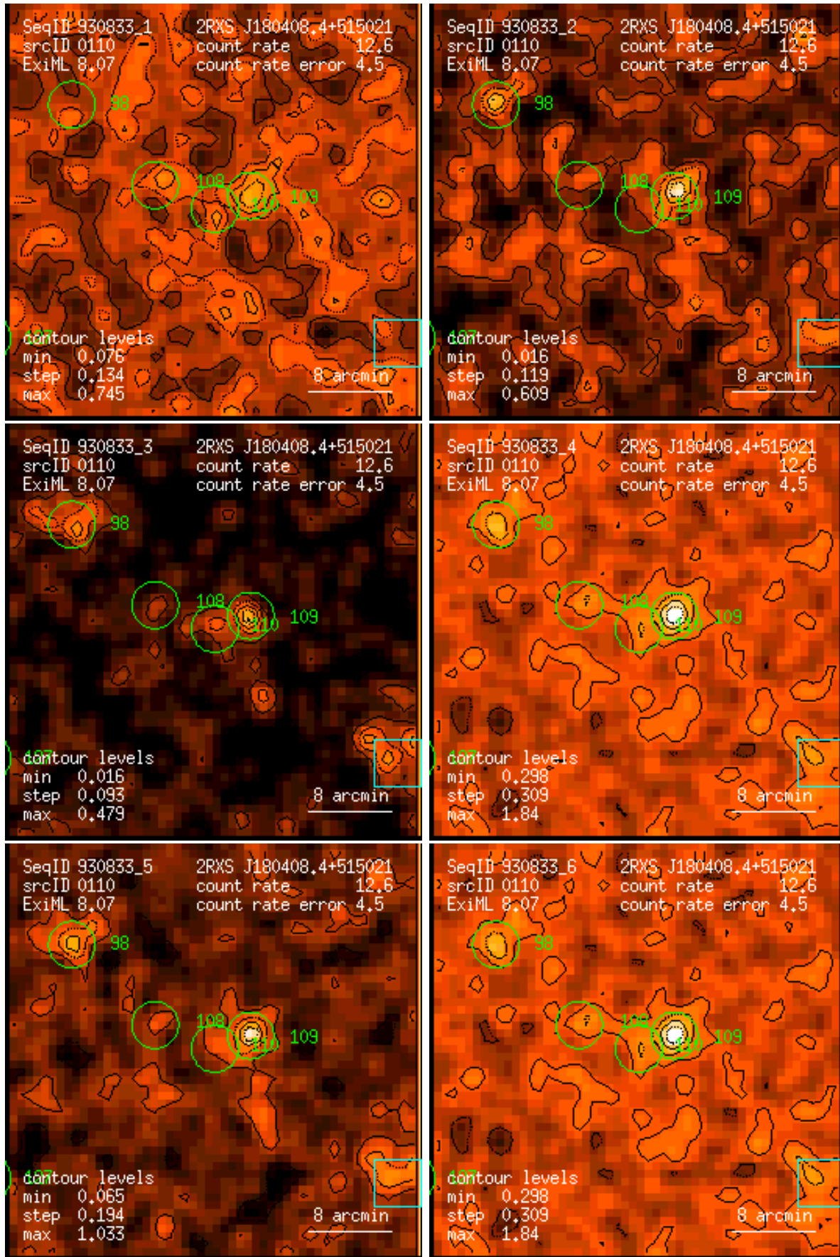
Figure 110: RASS 930833: detection 0110: band rate images, Gaussian filter: (1) PSPC channels 11 – 41, (2) 52 – 90, (3) 91 – 201, (4) 11 – 235, (5) 52 – 201, (6) 11 – 201. Broad band rates in counts/ks. Band rate contour levels in counts/ks/arcmin 2 .
