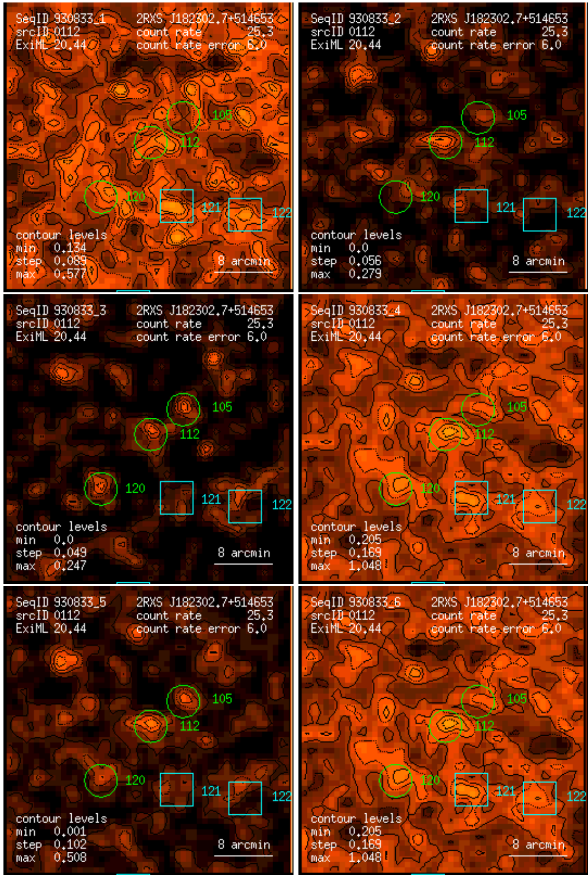
Figure 112: RASS 930833: detection 0112: band rate images, Gaussian filter: (1) PSPC channels 11 – 41, (2) 52 – 90, (3) 91 – 201, (4) 11 – 235, (5) 52 – 201, (6) 11 – 201. Broad band rates in counts/ks. Band rate contour levels in counts/ks/arcmin 2 .
