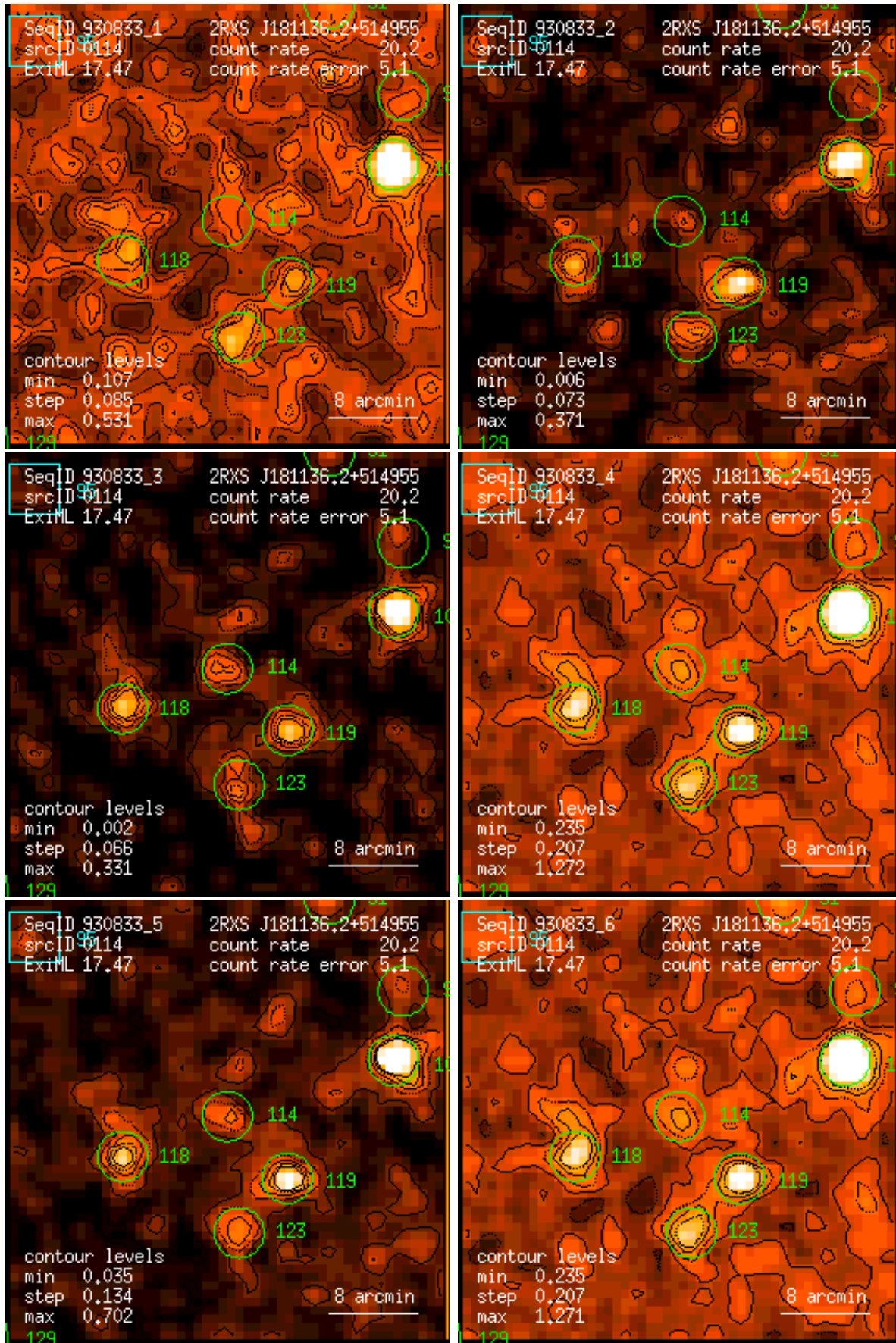
Figure 114: RASS 930833: detection 0114: band rate images, Gaussian filter: (1) PSPC channels 11 – 41, (2) 52 – 90, (3) 91 – 201, (4) 11 – 235, (5) 52 – 201, (6) 11 – 201. Broad band rates in counts/ks. Band rate contour levels in counts/ks/arcmin 2 .
