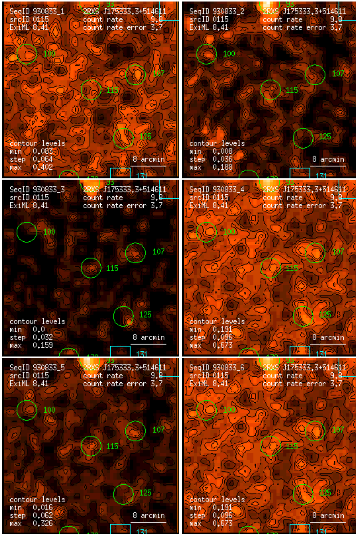
Figure 115: RASS 930833: detection 0115: band rate images, Gaussian filter: (1) PSPC channels 11 – 41, (2) 52 – 90, (3) 91 – 201, (4) 11 – 235, (5) 52 – 201, (6) 11 – 201. Broad band rates in counts/ks. Band rate contour levels in counts/ks/arcmin 2 .
