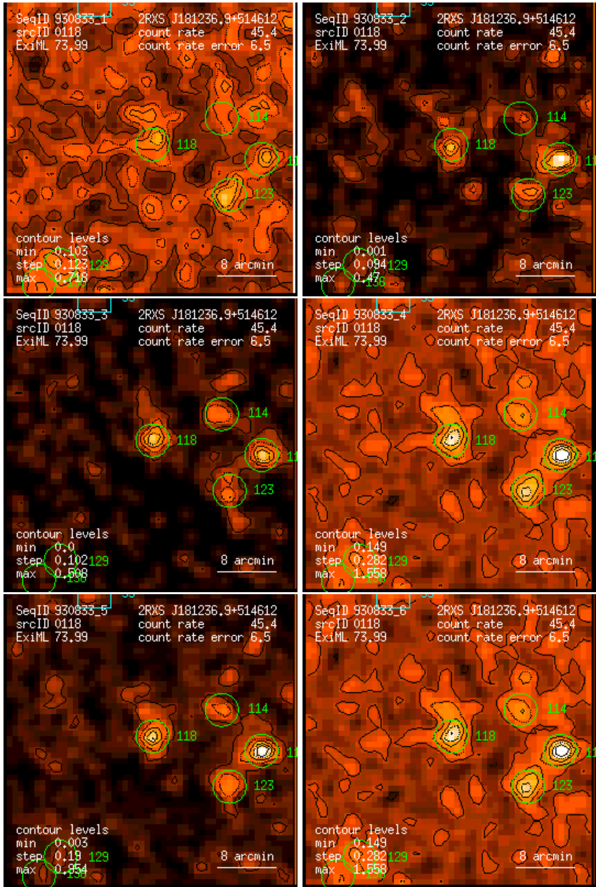
Figure 118: RASS 930833: detection 0118: band rate images, Gaussian filter: (1) PSPC channels 11 – 41, (2) 52 – 90, (3) 91 – 201, (4) 11 – 235, (5) 52 – 201, (6) 11 – 201. Broad band rates in counts/ks. Band rate contour levels in counts/ks/arcmin 2 .
