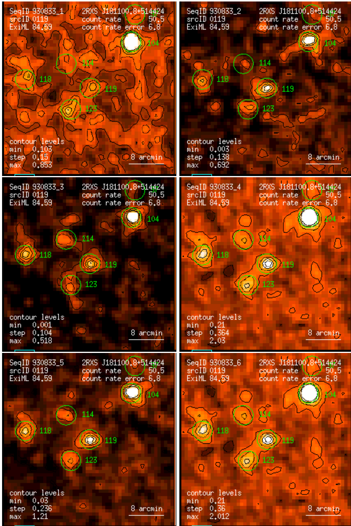
Figure 119: RASS 930833: detection 0119: band rate images, Gaussian filter: (1) PSPC channels 11 – 41, (2) 52 – 90, (3) 91 – 201, (4) 11 – 235, (5) 52 – 201, (6) 11 – 201. Broad band rates in counts/ks. Band rate contour levels in counts/ks/arcmin 2 .
