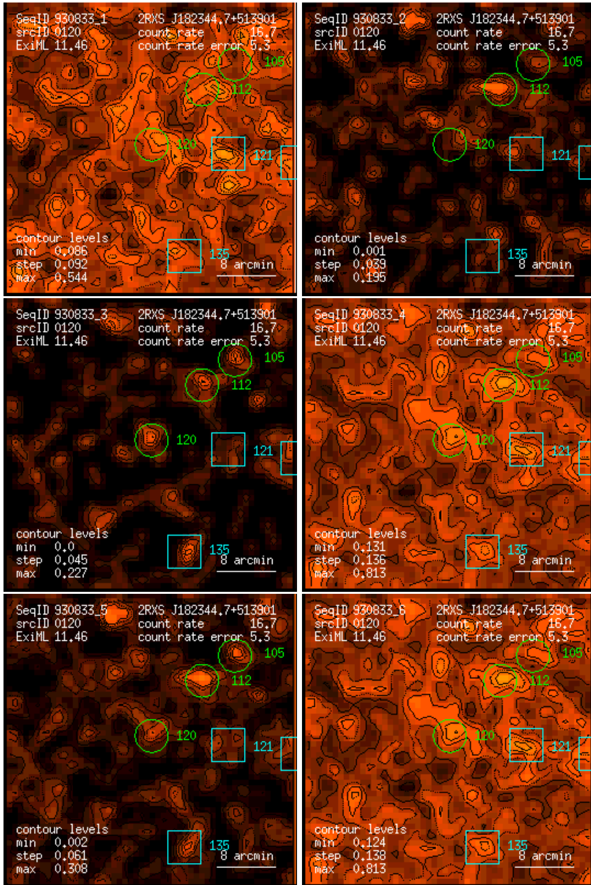
Figure 120: RASS 930833: detection 0120: band rate images, Gaussian filter: (1) PSPC channels 11 – 41, (2) 52 – 90, (3) 91 – 201, (4) 11 – 235, (5) 52 – 201, (6) 11 – 201. Broad band rates in counts/ks. Band rate contour levels in counts/ks/arcmin 2 .
