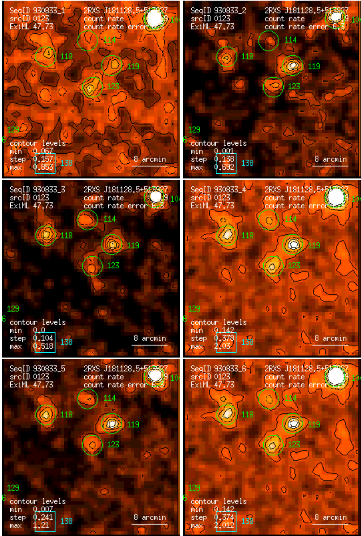
Figure 123: RASS 930833: detection 0123: band rate images, Gaussian filter: (1) PSPC channels 11 – 41, (2) 52 – 90, (3) 91 – 201, (4) 11 – 235, (5) 52 – 201, (6) 11 – 201. Broad band rates in counts/ks. Band rate contour levels in counts/ks/arcmin 2 .
