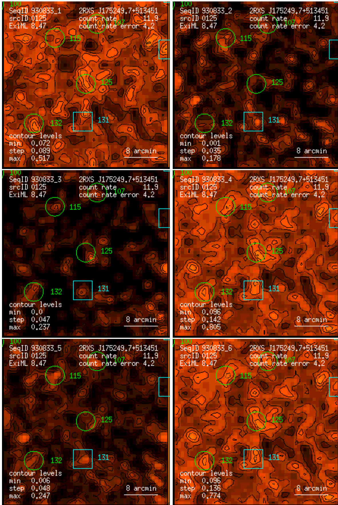
Figure 125: RASS 930833: detection 0125: band rate images, Gaussian filter: (1) PSPC channels 11 – 41, (2) 52 – 90, (3) 91 – 201, (4) 11 – 235, (5) 52 – 201, (6) 11 – 201. Broad band rates in counts/ks. Band rate contour levels in counts/ks/arcmin 2 .
