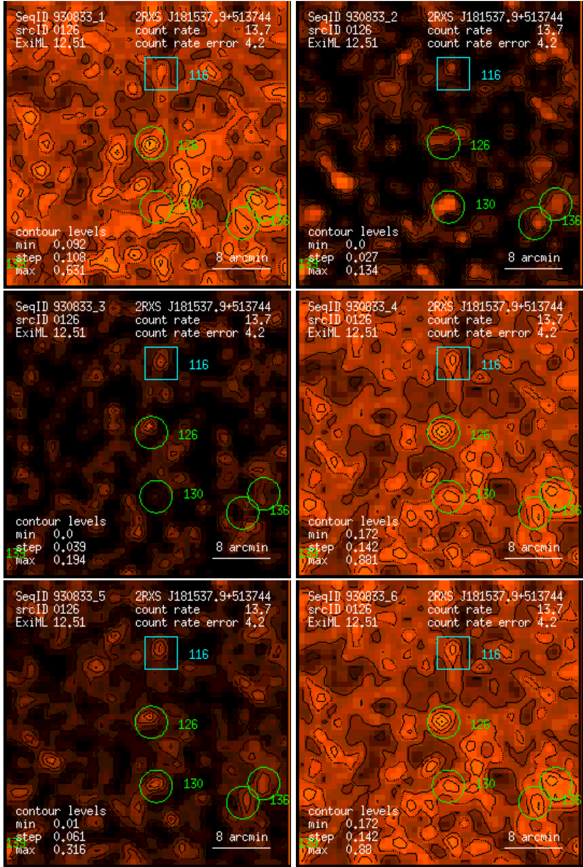
Figure 126: RASS 930833: detection 0126: band rate images, Gaussian filter: (1) PSPC channels 11 – 41, (2) 52 – 90, (3) 91 – 201, (4) 11 – 235, (5) 52 – 201, (6) 11 – 201. Broad band rates in counts/ks. Band rate contour levels in counts/ks/arcmin 2 .
