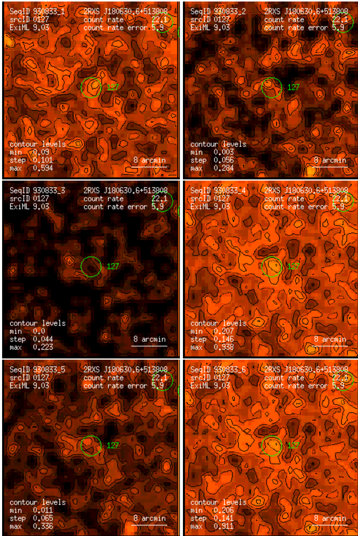
Figure 127: RASS 930833: detection 0127: band rate images, Gaussian filter: (1) PSPC channels 11 – 41, (2) 52 – 90, (3) 91 – 201, (4) 11 – 235, (5) 52 – 201, (6) 11 – 201. Broad band rates in counts/ks. Band rate contour levels in counts/ks/arcmin 2 .
