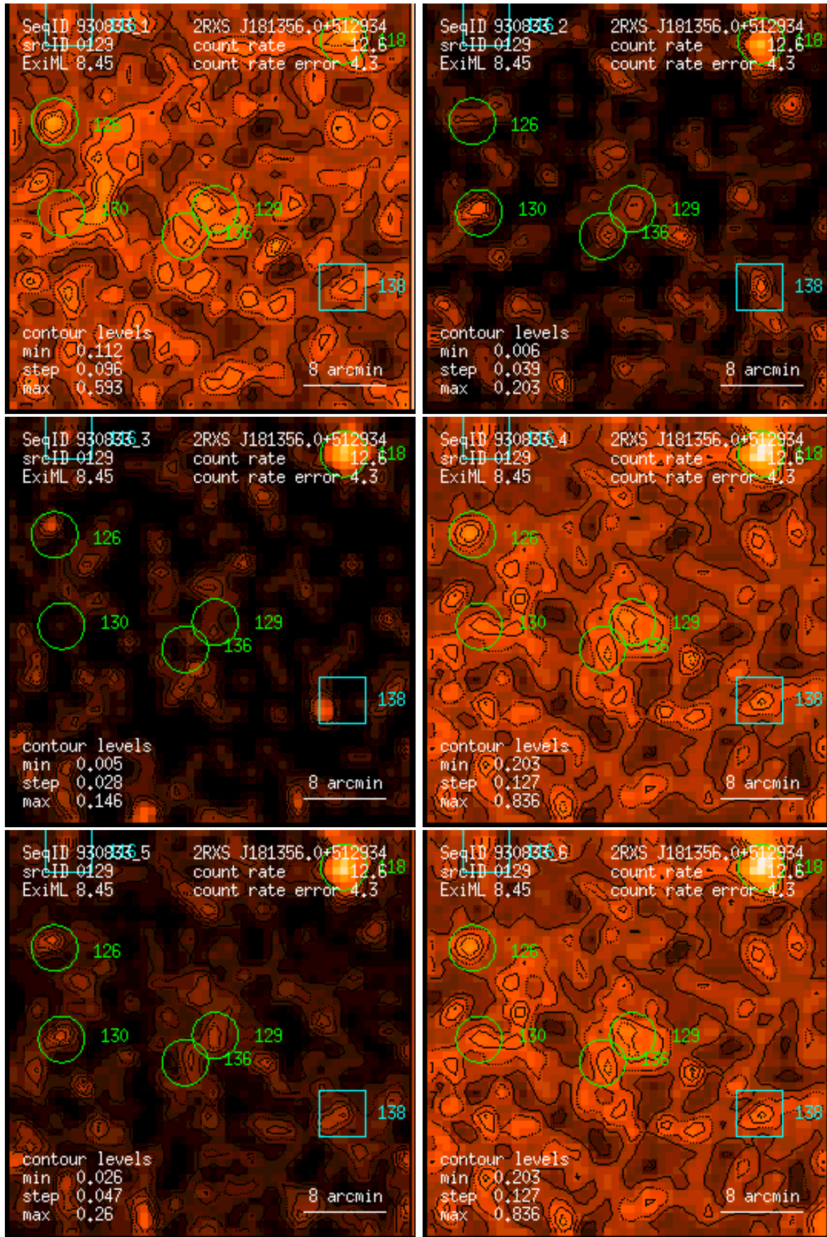
Figure 129: RASS 930833: detection 0129: band rate images, Gaussian filter: (1) PSPC channels 11 – 41, (2) 52 – 90, (3) 91 – 201, (4) 11 – 235, (5) 52 – 201, (6) 11 – 201. Broad band rates in counts/ks. Band rate contour levels in counts/ks/arcmin 2 .
