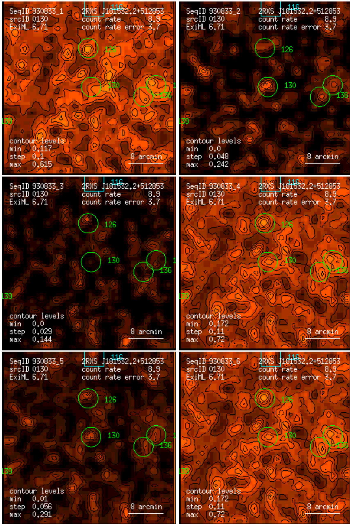
Figure 130: RASS 930833: detection 0130: band rate images, Gaussian filter: (1) PSPC channels 11 – 41, (2) 52 – 90, (3) 91 – 201, (4) 11 – 235, (5) 52 – 201, (6) 11 – 201. Broad band rates in counts/ks. Band rate contour levels in counts/ks/arcmin 2 .
