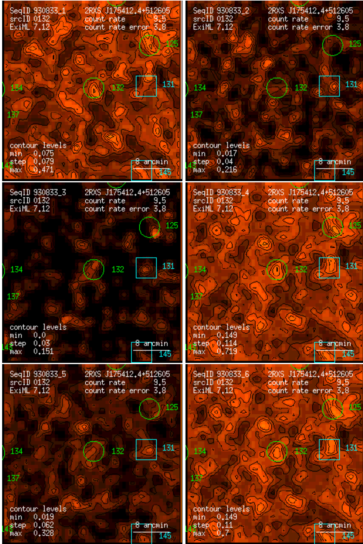
Figure 132: RASS 930833: detection 0132: band rate images, Gaussian filter: (1) PSPC channels 11 – 41, (2) 52 – 90, (3) 91 – 201, (4) 11 – 235, (5) 52 – 201, (6) 11 – 201. Broad band rates in counts/ks. Band rate contour levels in counts/ks/arcmin 2 .
