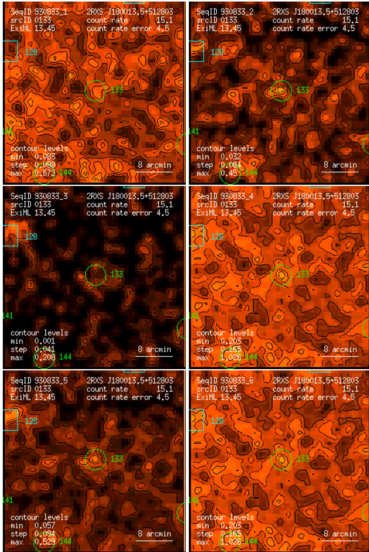
Figure 133: RASS 930833: detection 0133: band rate images, Gaussian filter: (1) PSPC channels 11 – 41, (2) 52 – 90, (3) 91 – 201, (4) 11 – 235, (5) 52 – 201, (6) 11 – 201. Broad band rates in counts/ks. Band rate contour levels in counts/ks/arcmin 2 .
