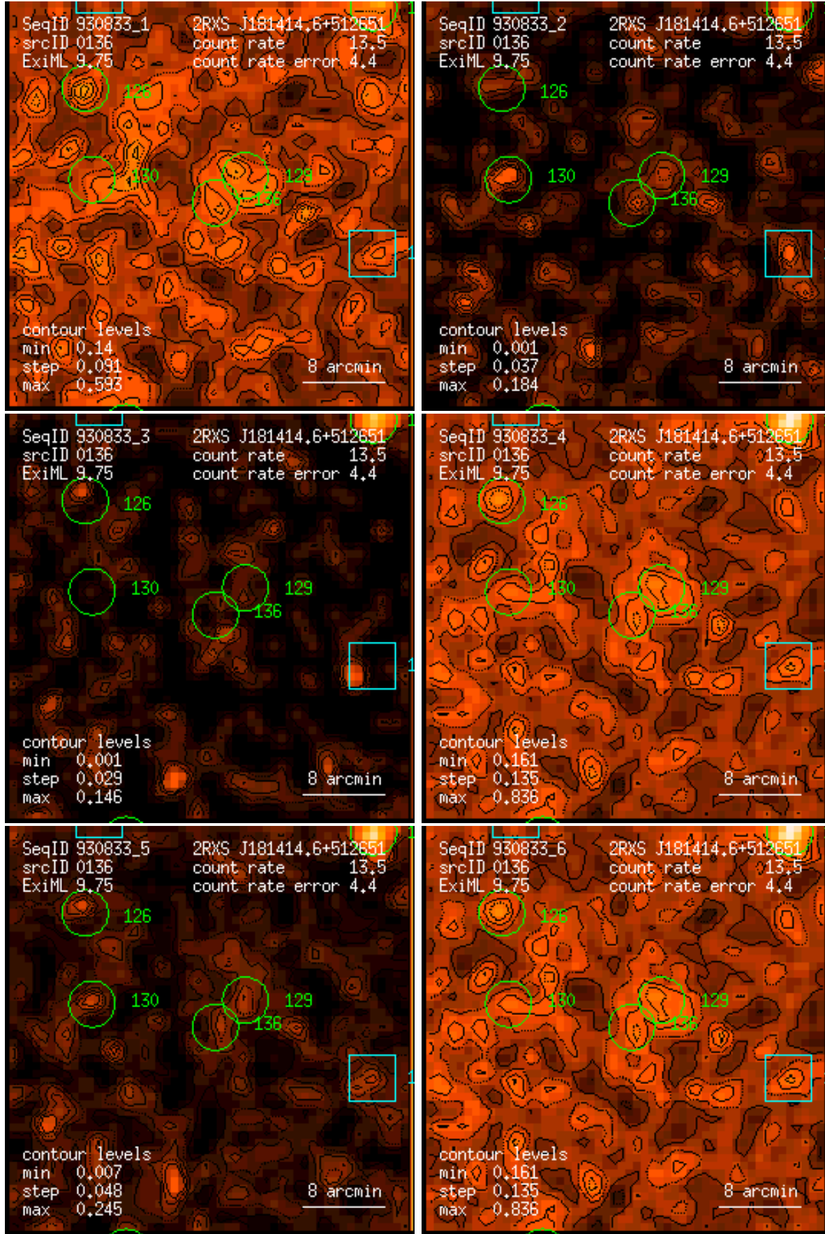
Figure 136: RASS 930833: detection 0136: band rate images, Gaussian filter: (1) PSPC channels 11 – 41, (2) 52 – 90, (3) 91 – 201, (4) 11 – 235, (5) 52 – 201, (6) 11 – 201. Broad band rates in counts/ks. Band rate contour levels in counts/ks/arcmin 2 .
