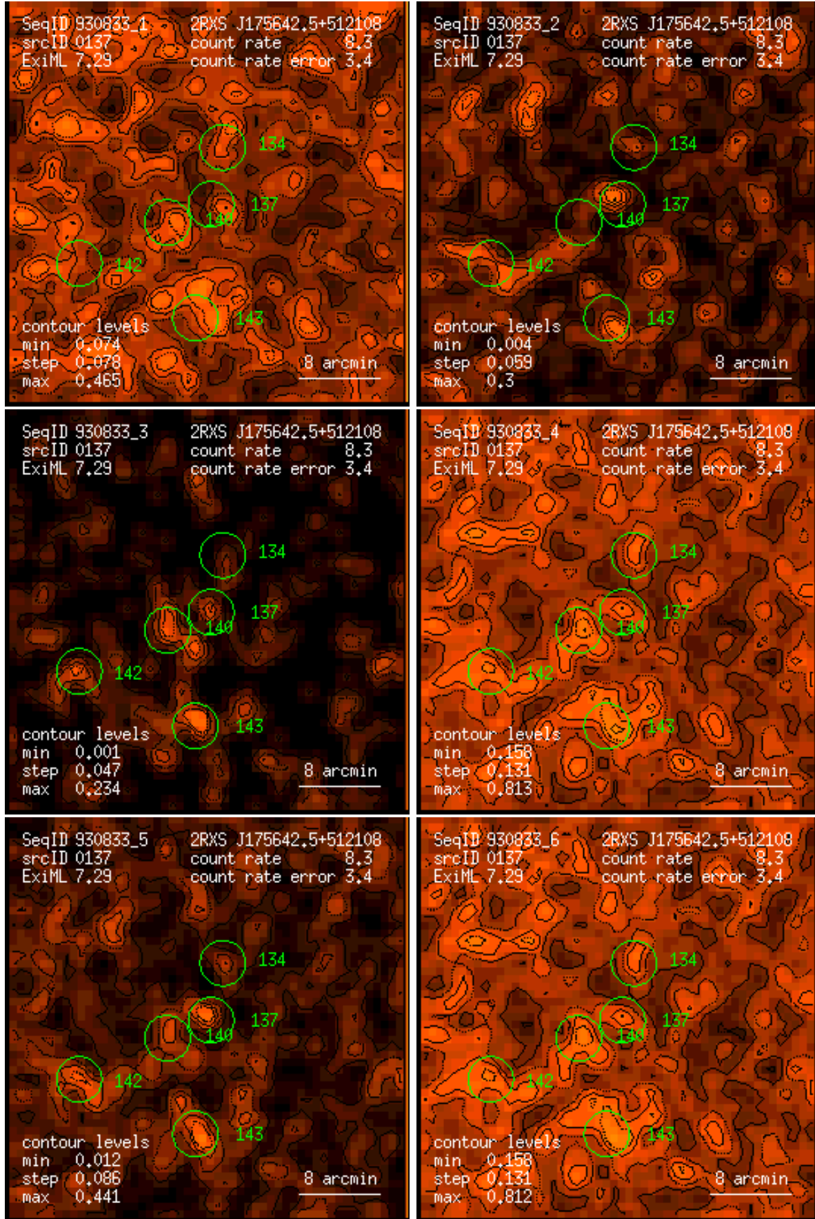
Figure 137: RASS 930833: detection 0137: band rate images, Gaussian filter: (1) PSPC channels 11 – 41, (2) 52 – 90, (3) 91 – 201, (4) 11 – 235, (5) 52 – 201, (6) 11 – 201. Broad band rates in counts/ks. Band rate contour levels in counts/ks/arcmin 2 .
