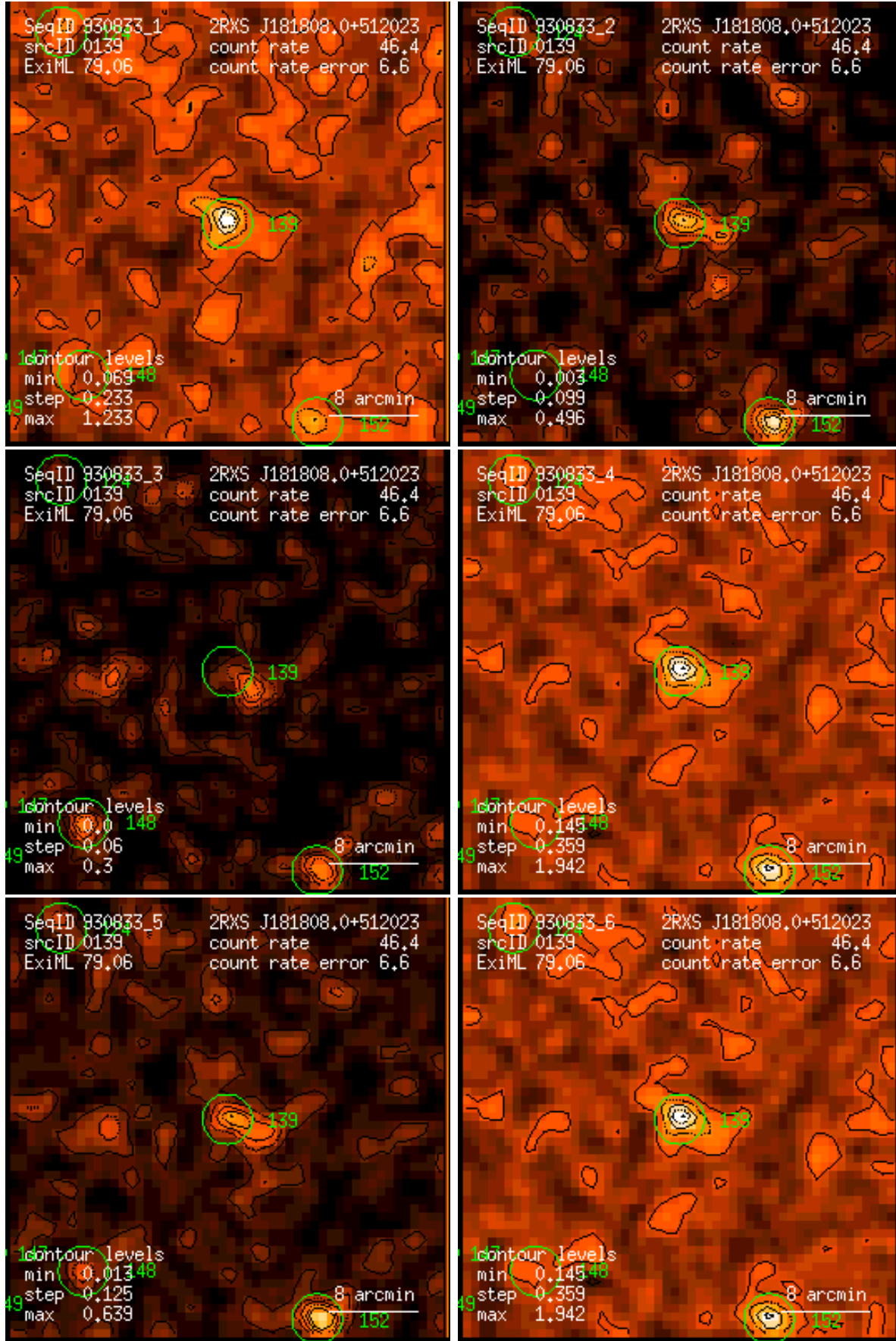
Figure 139: RASS 930833: detection 0139: band rate images, Gaussian filter: (1) PSPC channels 11 – 41, (2) 52 – 90, (3) 91 – 201, (4) 11 – 235, (5) 52 – 201, (6) 11 – 201. Broad band rates in counts/ks. Band rate contour levels in counts/ks/arcmin 2 .
