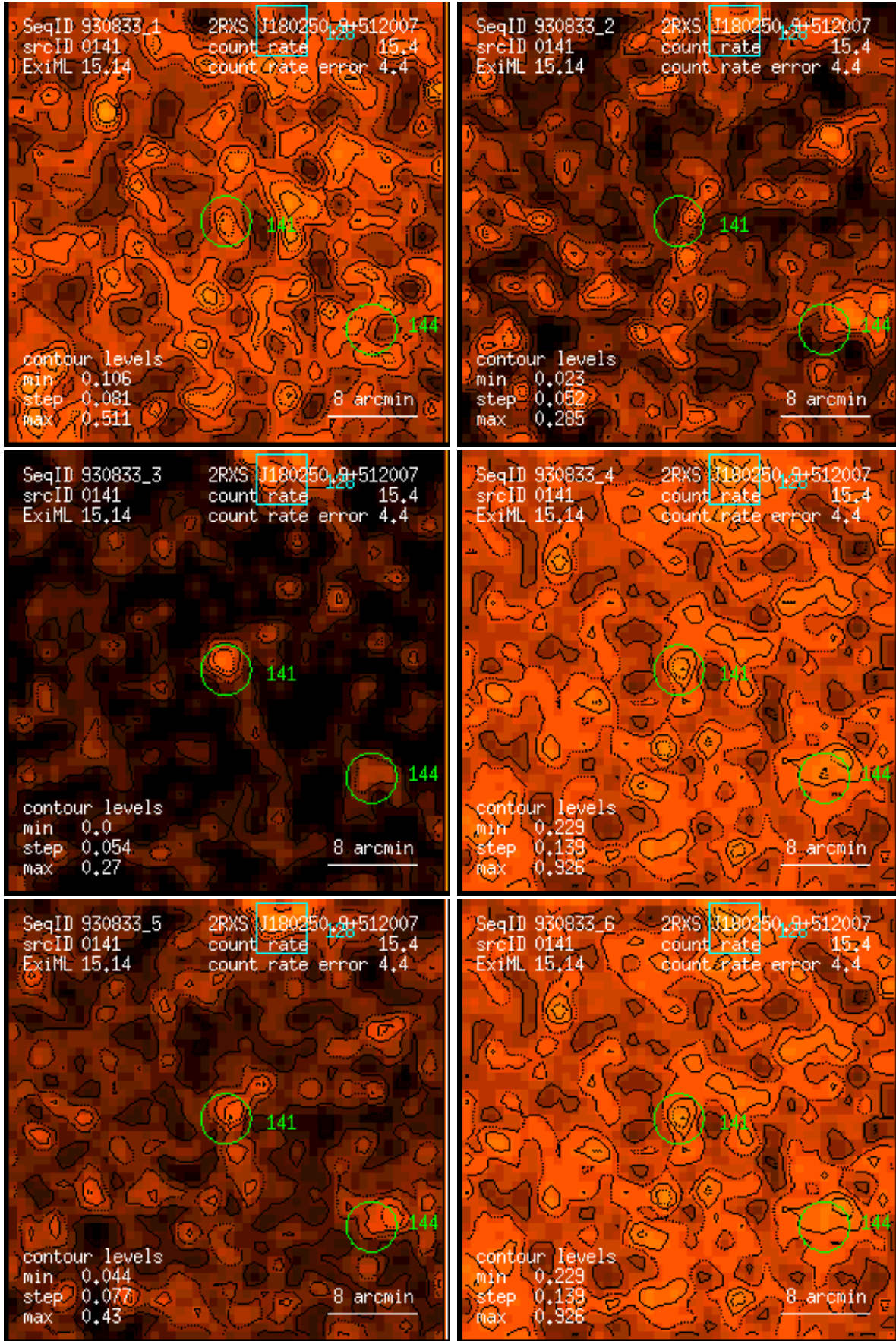
Figure 141: RASS 930833: detection 0141: band rate images, Gaussian filter: (1) PSPC channels 11 – 41, (2) 52 – 90, (3) 91 – 201, (4) 11 – 235, (5) 52 – 201, (6) 11 – 201. Broad band rates in counts/ks. Band rate contour levels in counts/ks/arcmin 2 .
