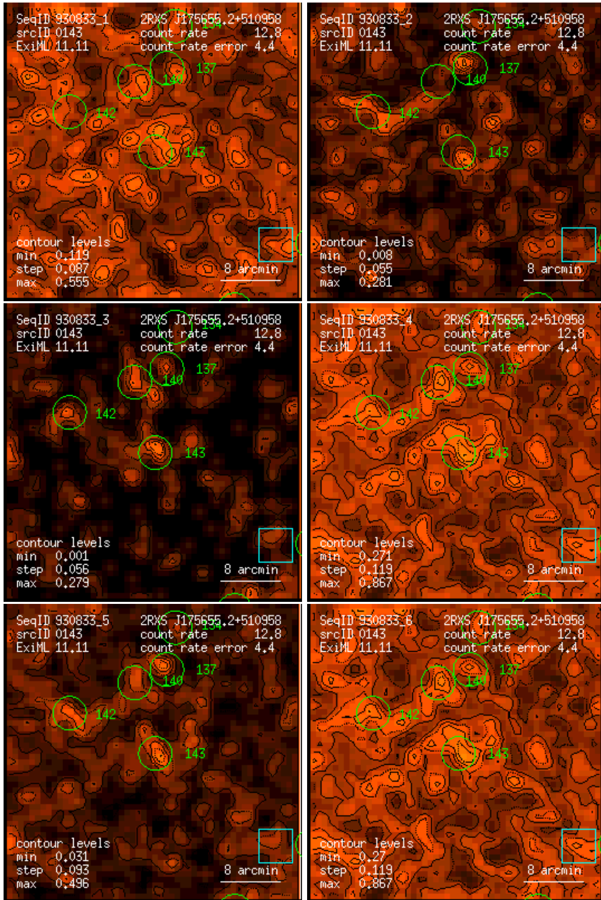
Figure 143: RASS 930833: detection 0143: band rate images, Gaussian filter: (1) PSPC channels 11 – 41, (2) 52 – 90, (3) 91 – 201, (4) 11 – 235, (5) 52 – 201, (6) 11 – 201. Broad band rates in counts/ks. Band rate contour levels in counts/ks/arcmin 2 .
