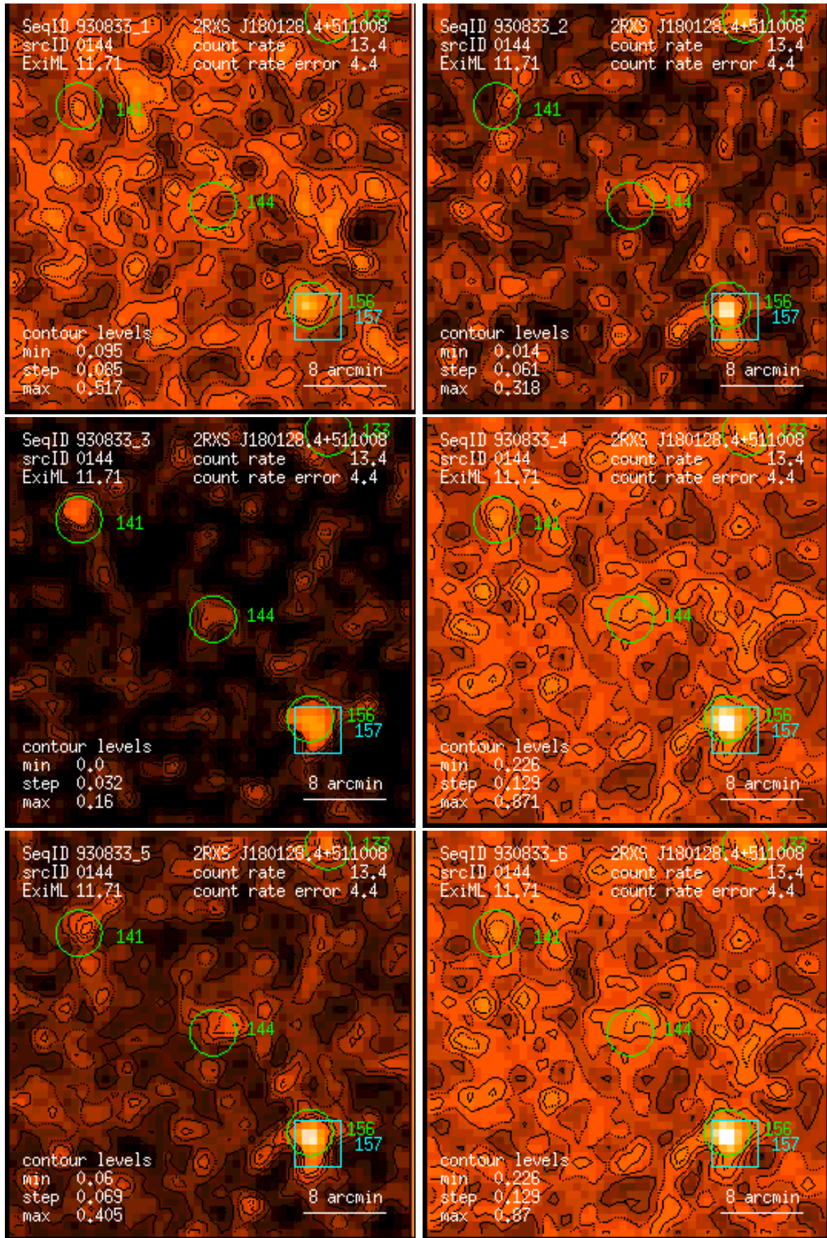
Figure 144: RASS 930833: detection 0144: band rate images, Gaussian filter: (1) PSPC channels 11 – 41, (2) 52 – 90, (3) 91 – 201, (4) 11 – 235, (5) 52 – 201, (6) 11 – 201. Broad band rates in counts/ks. Band rate contour levels in counts/ks/arcmin 2 .
