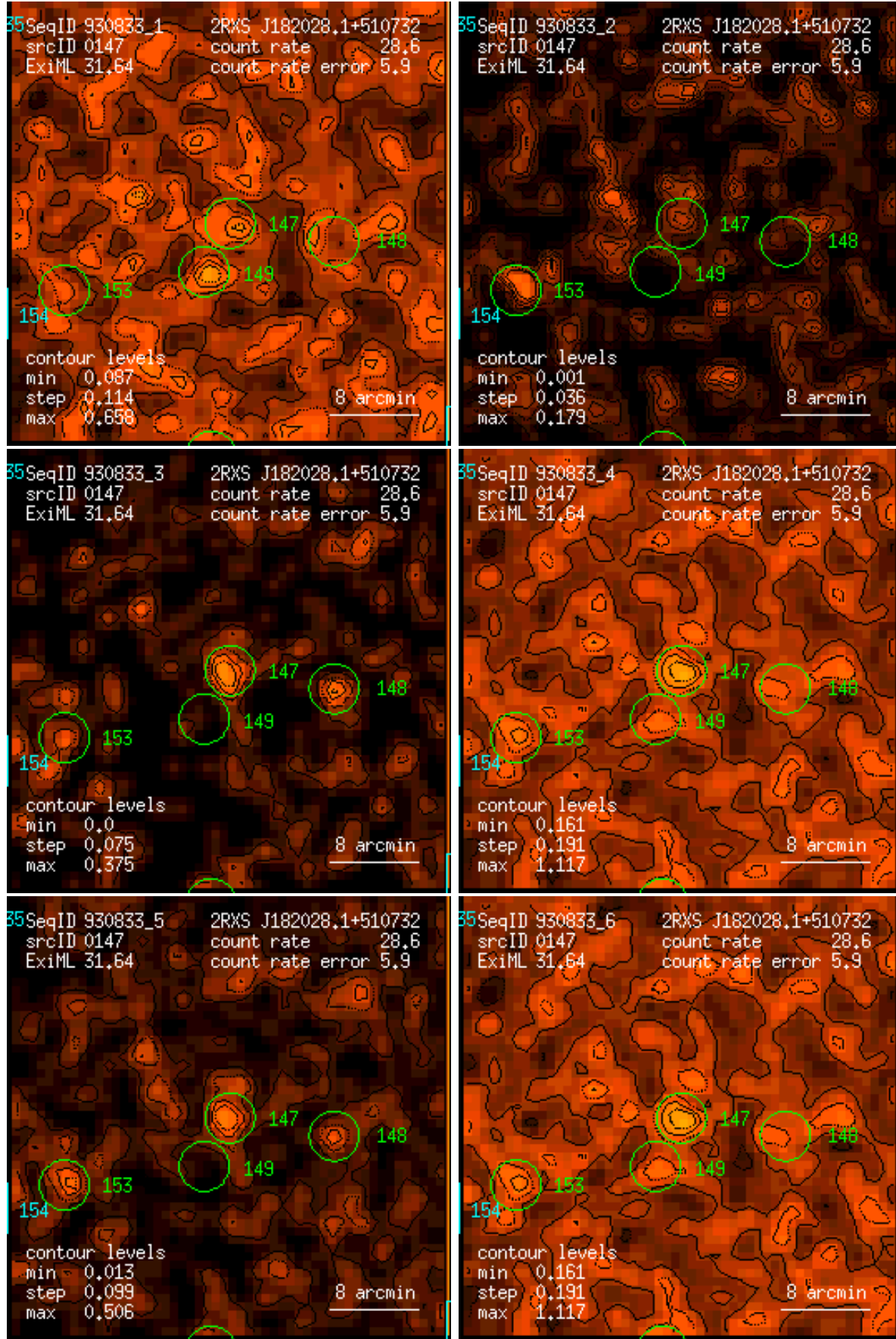
Figure 147: RASS 930833: detection 0147: band rate images, Gaussian filter: (1) PSPC channels 11 – 41, (2) 52 – 90, (3) 91 – 201, (4) 11 – 235, (5) 52 – 201, (6) 11 – 201. Broad band rates in counts/ks. Band rate contour levels in counts/ks/arcmin 2 .
