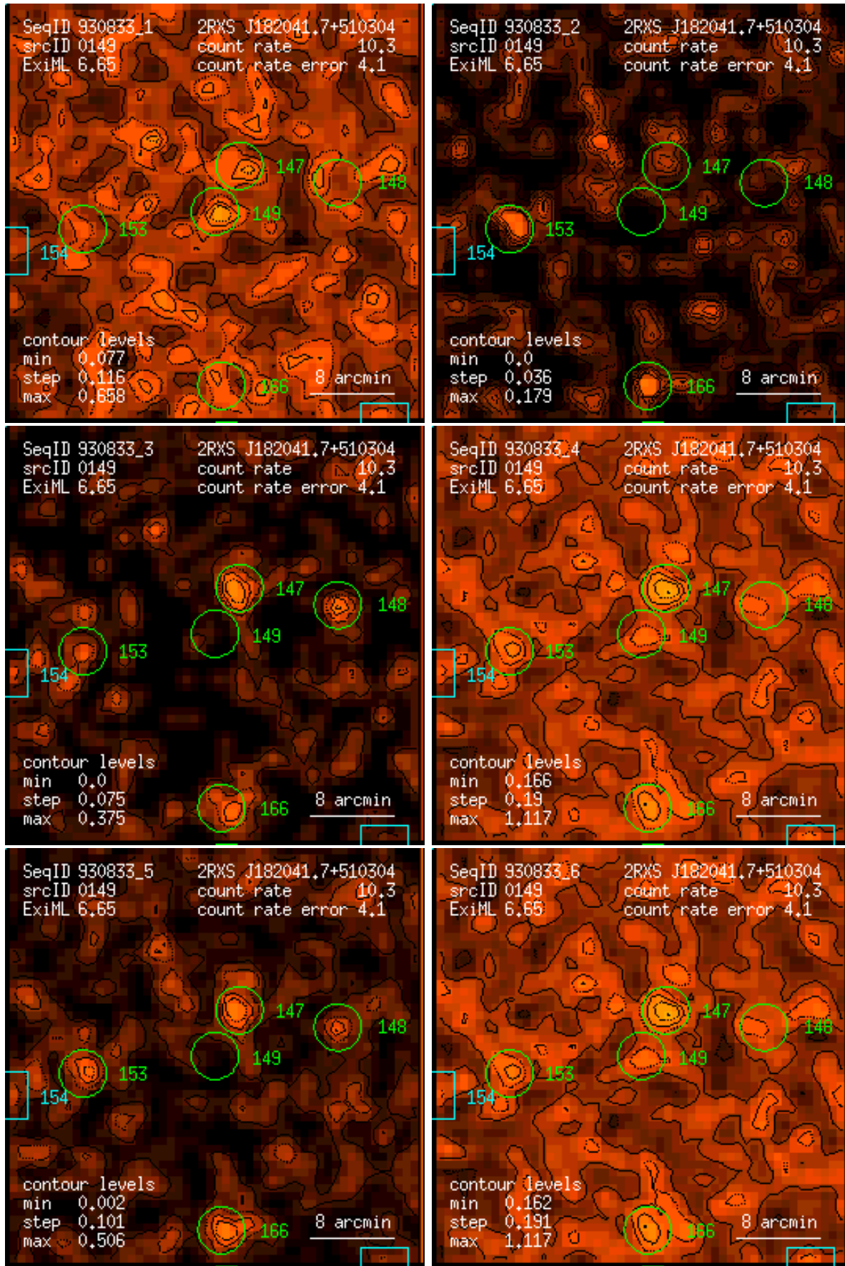
Figure 149: RASS 930833: detection 0149: band rate images, Gaussian filter: (1) PSPC channels 11 – 41, (2) 52 – 90, (3) 91 – 201, (4) 11 – 235, (5) 52 – 201, (6) 11 – 201. Broad band rates in counts/ks. Band rate contour levels in counts/ks/arcmin 2 .
