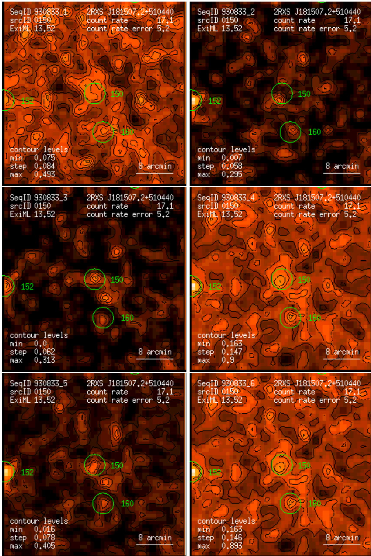
Figure 150: RASS 930833: detection 0150: band rate images, Gaussian filter: (1) PSPC channels 11 – 41, (2) 52 – 90, (3) 91 – 201, (4) 11 – 235, (5) 52 – 201, (6) 11 – 201. Broad band rates in counts/ks. Band rate contour levels in counts/ks/arcmin 2 .
