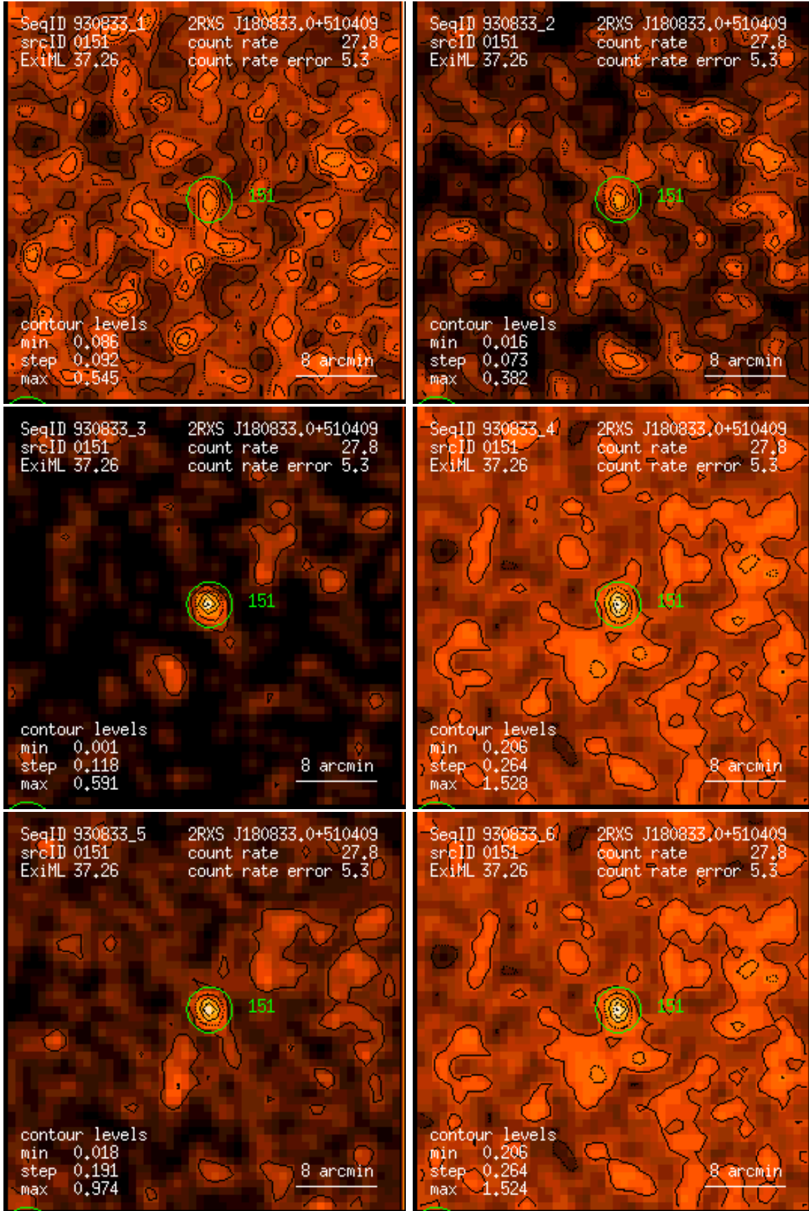
Figure 151: RASS 930833: detection 0151: band rate images, Gaussian filter: (1) PSPC channels 11 – 41, (2) 52 – 90, (3) 91 – 201, (4) 11 – 235, (5) 52 – 201, (6) 11 – 201. Broad band rates in counts/ks. Band rate contour levels in counts/ks/arcmin 2 .
