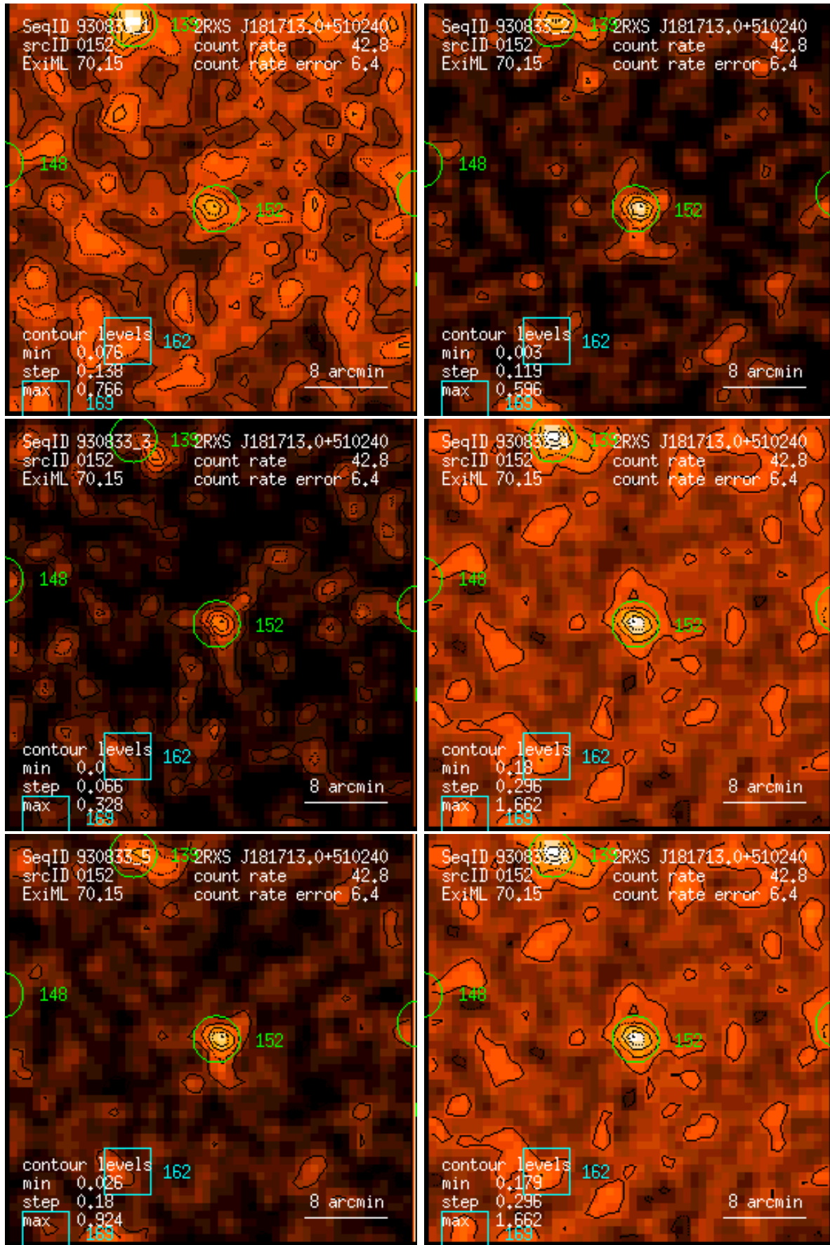
Figure 152: RASS 930833: detection 0152: band rate images, Gaussian filter: (1) PSPC channels 11 – 41, (2) 52 – 90, (3) 91 – 201, (4) 11 – 235, (5) 52 – 201, (6) 11 – 201. Broad band rates in counts/ks. Band rate contour levels in counts/ks/arcmin 2 .
