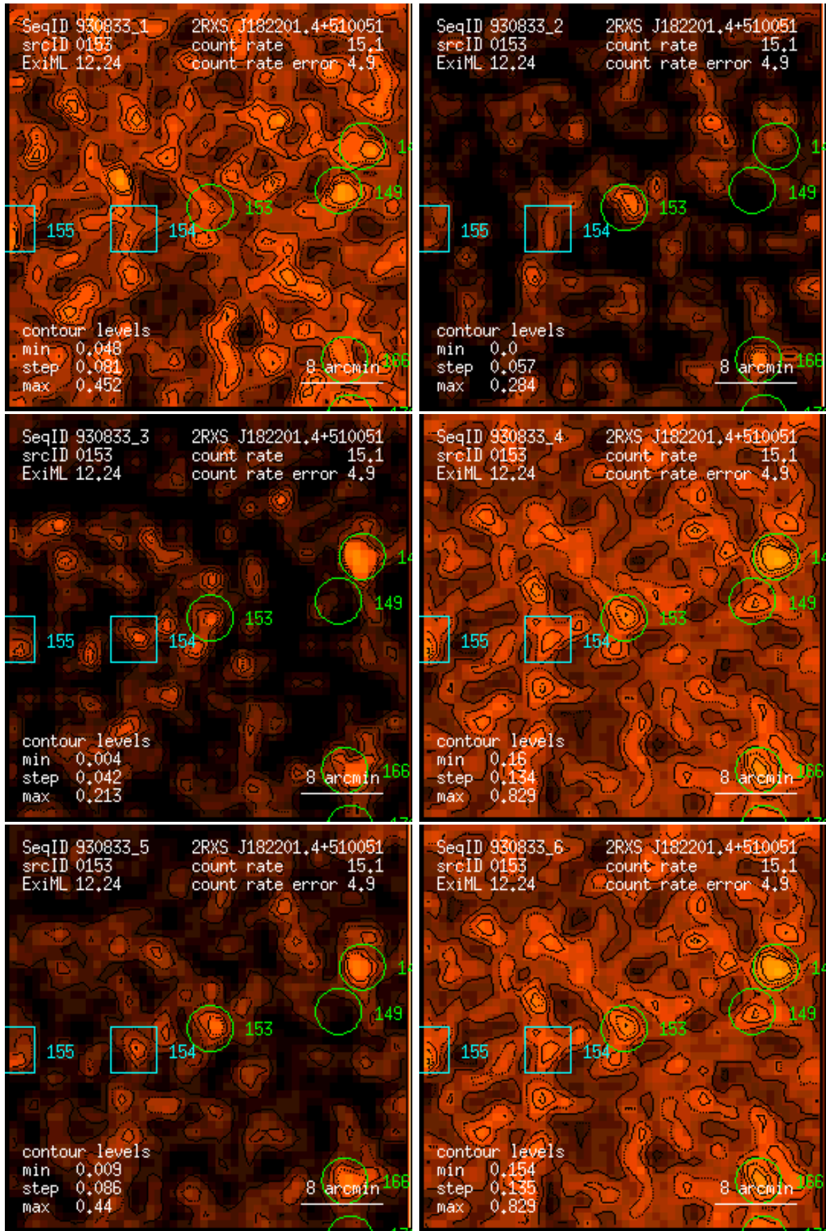
Figure 153: RASS 930833: detection 0153: band rate images, Gaussian filter: (1) PSPC channels 11 – 41, (2) 52 – 90, (3) 91 – 201, (4) 11 – 235, (5) 52 – 201, (6) 11 – 201. Broad band rates in counts/ks. Band rate contour levels in counts/ks/arcmin 2 .
