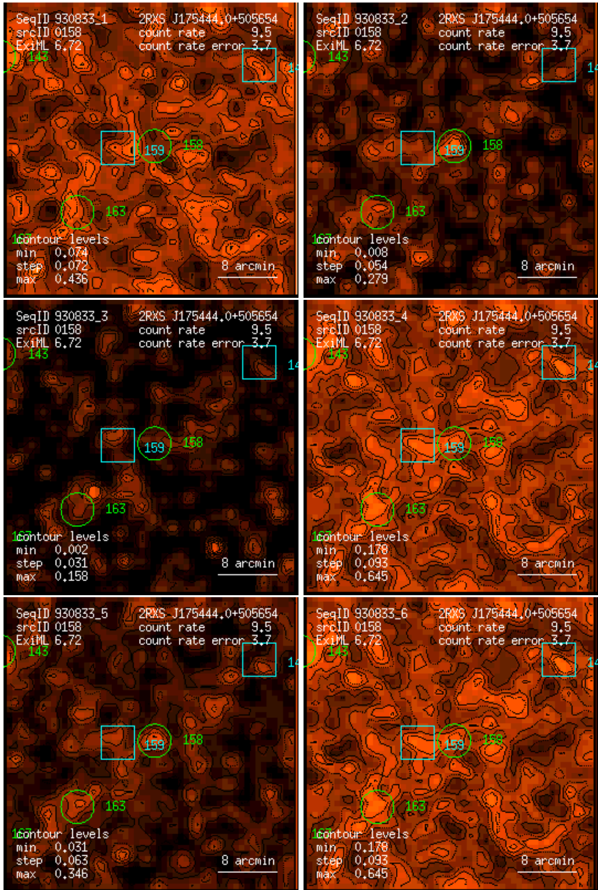
Figure 158: RASS 930833: detection 0158: band rate images, Gaussian filter: (1) PSPC channels 11 – 41, (2) 52 – 90, (3) 91 – 201, (4) 11 – 235, (5) 52 – 201, (6) 11 – 201. Broad band rates in counts/ks. Band rate contour levels in counts/ks/arcmin 2 .
