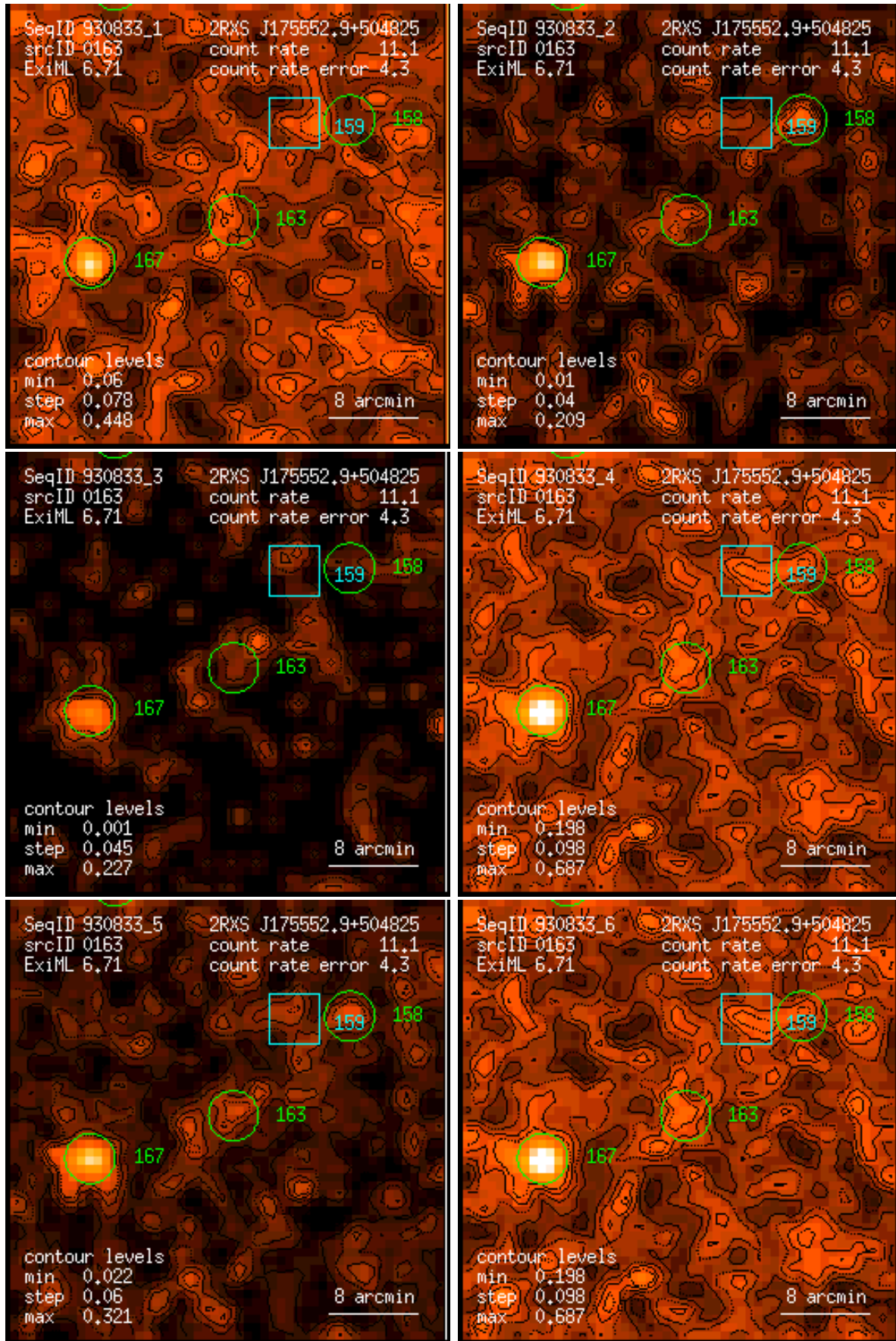
Figure 163: RASS 930833: detection 0163: band rate images, Gaussian filter: (1) PSPC channels 11 – 41, (2) 52 – 90, (3) 91 – 201, (4) 11 – 235, (5) 52 – 201, (6) 11 – 201. Broad band rates in counts/ks. Band rate contour levels in counts/ks/arcmin 2 .
