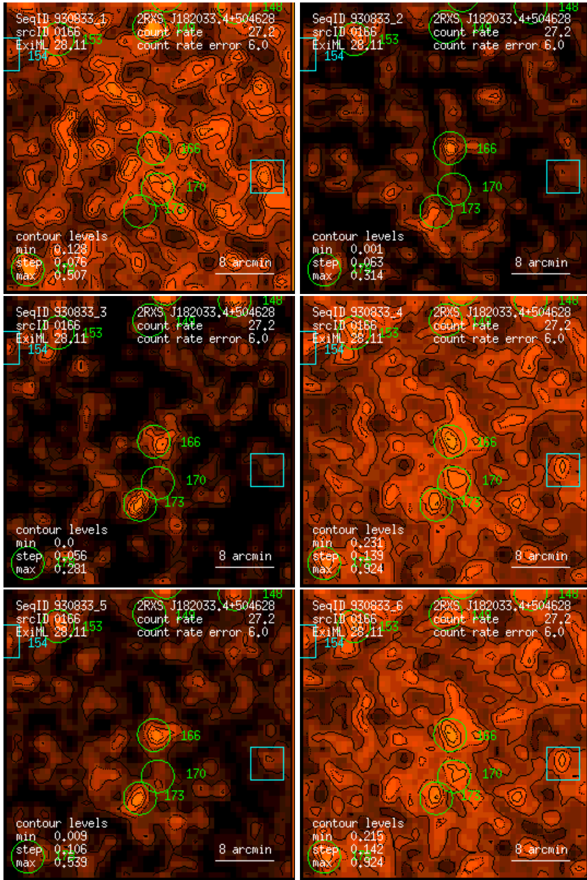
Figure 166: RASS 930833: detection 0166: band rate images, Gaussian filter: (1) PSPC channels 11 – 41, (2) 52 – 90, (3) 91 – 201, (4) 11 – 235, (5) 52 – 201, (6) 11 – 201. Broad band rates in counts/ks. Band rate contour levels in counts/ks/arcmin 2 .
