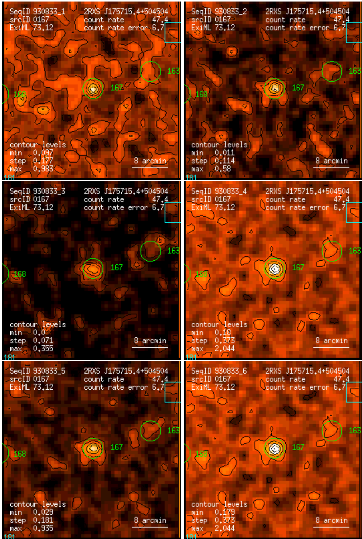
Figure 167: RASS 930833: detection 0167: band rate images, Gaussian filter: (1) PSPC channels 11 – 41, (2) 52 – 90, (3) 91 – 201, (4) 11 – 235, (5) 52 – 201, (6) 11 – 201. Broad band rates in counts/ks. Band rate contour levels in counts/ks/arcmin 2 .
