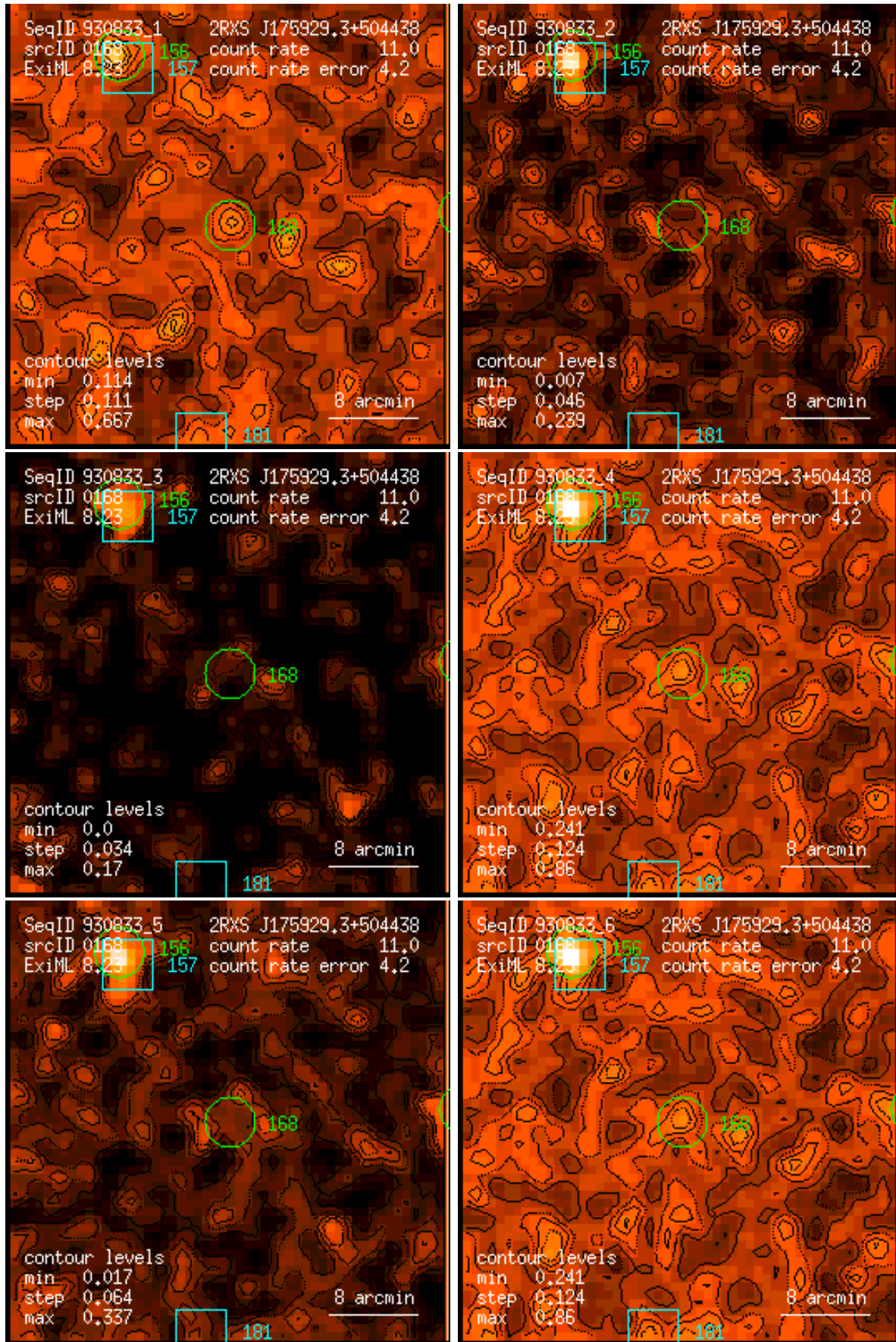
Figure 168: RASS 930833: detection 0168: band rate images, Gaussian filter: (1) PSPC channels 11 – 41, (2) 52 – 90, (3) 91 – 201, (4) 11 – 235, (5) 52 – 201, (6) 11 – 201. Broad band rates in counts/ks. Band rate contour levels in counts/ks/arcmin 2 .
