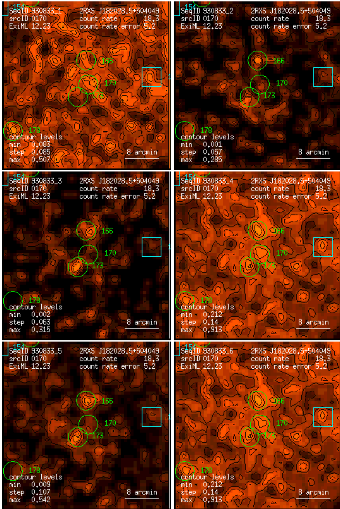
Figure 170: RASS 930833: detection 0170: band rate images, Gaussian filter: (1) PSPC channels 11 – 41, (2) 52 – 90, (3) 91 – 201, (4) 11 – 235, (5) 52 – 201, (6) 11 – 201. Broad band rates in counts/ks. Band rate contour levels in counts/ks/arcmin 2 .
