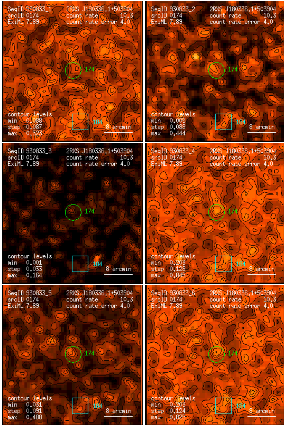
Figure 174: RASS 930833: detection 0174: band rate images, Gaussian filter: (1) PSPC channels 11 – 41, (2) 52 – 90, (3) 91 – 201, (4) 11 – 235, (5) 52 – 201, (6) 11 – 201. Broad band rates in counts/ks. Band rate contour levels in counts/ks/arcmin 2 .
