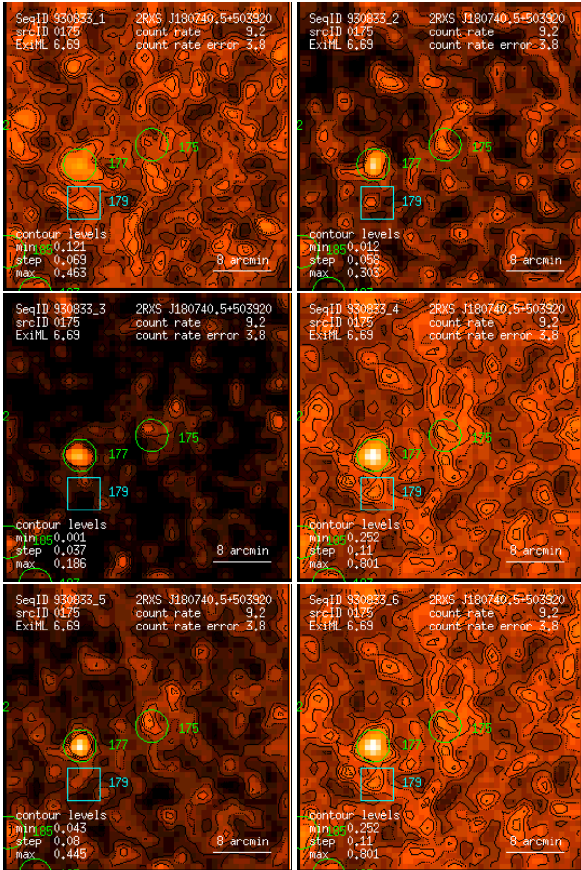
Figure 175: RASS 930833: detection 0175: band rate images, Gaussian filter: (1) PSPC channels 11 – 41, (2) 52 – 90, (3) 91 – 201, (4) 11 – 235, (5) 52 – 201, (6) 11 – 201. Broad band rates in counts/ks. Band rate contour levels in counts/ks/arcmin 2 .
