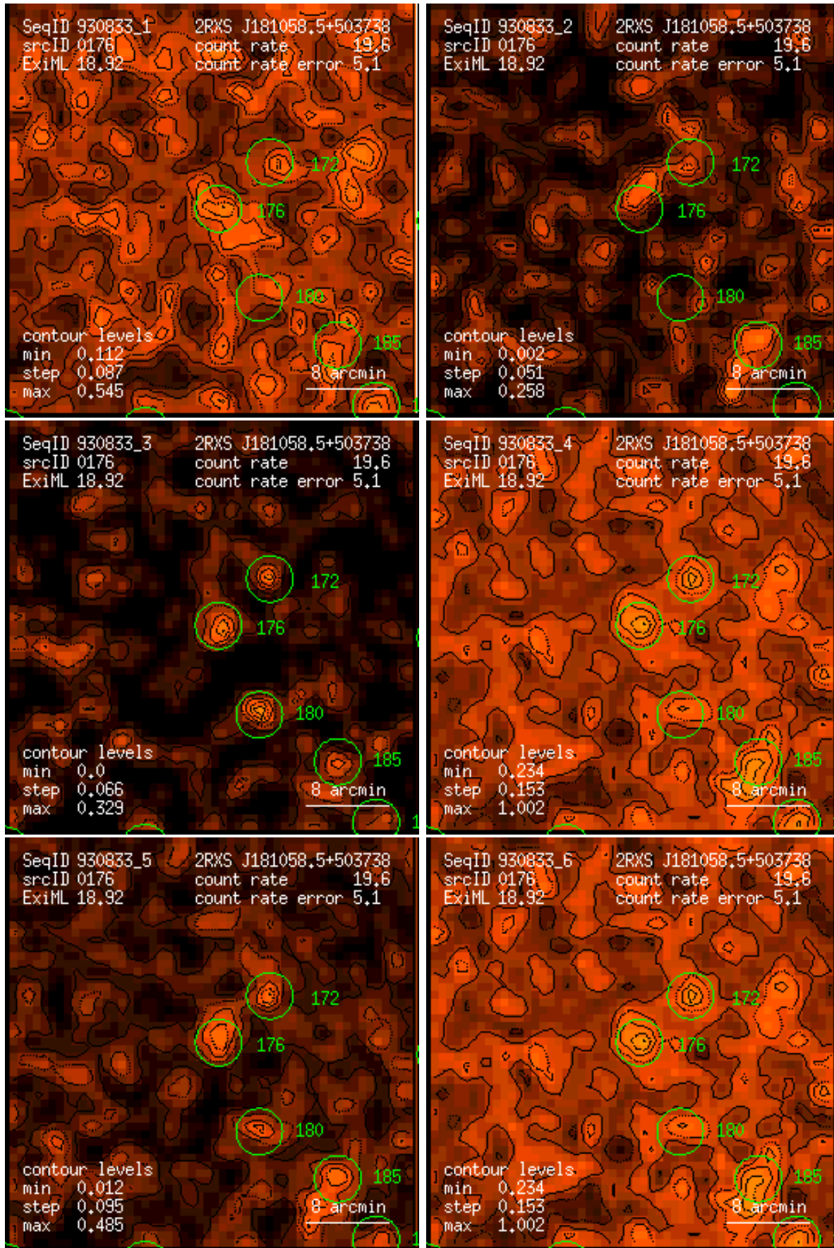
Figure 176: RASS 930833: detection 0176: band rate images, Gaussian filter: (1) PSPC channels 11 – 41, (2) 52 – 90, (3) 91 – 201, (4) 11 – 235, (5) 52 – 201, (6) 11 – 201. Broad band rates in counts/ks. Band rate contour levels in counts/ks/arcmin 2 .
