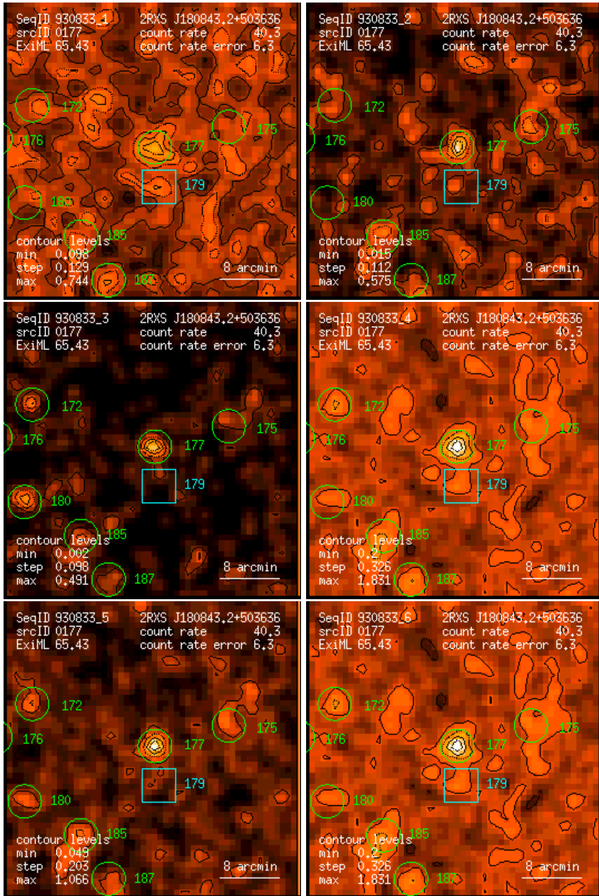
Figure 177: RASS 930833: detection 0177: band rate images, Gaussian filter: (1) PSPC channels 11 – 41, (2) 52 – 90, (3) 91 – 201, (4) 11 – 235, (5) 52 – 201, (6) 11 – 201. Broad band rates in counts/ks. Band rate contour levels in counts/ks/arcmin 2 .
